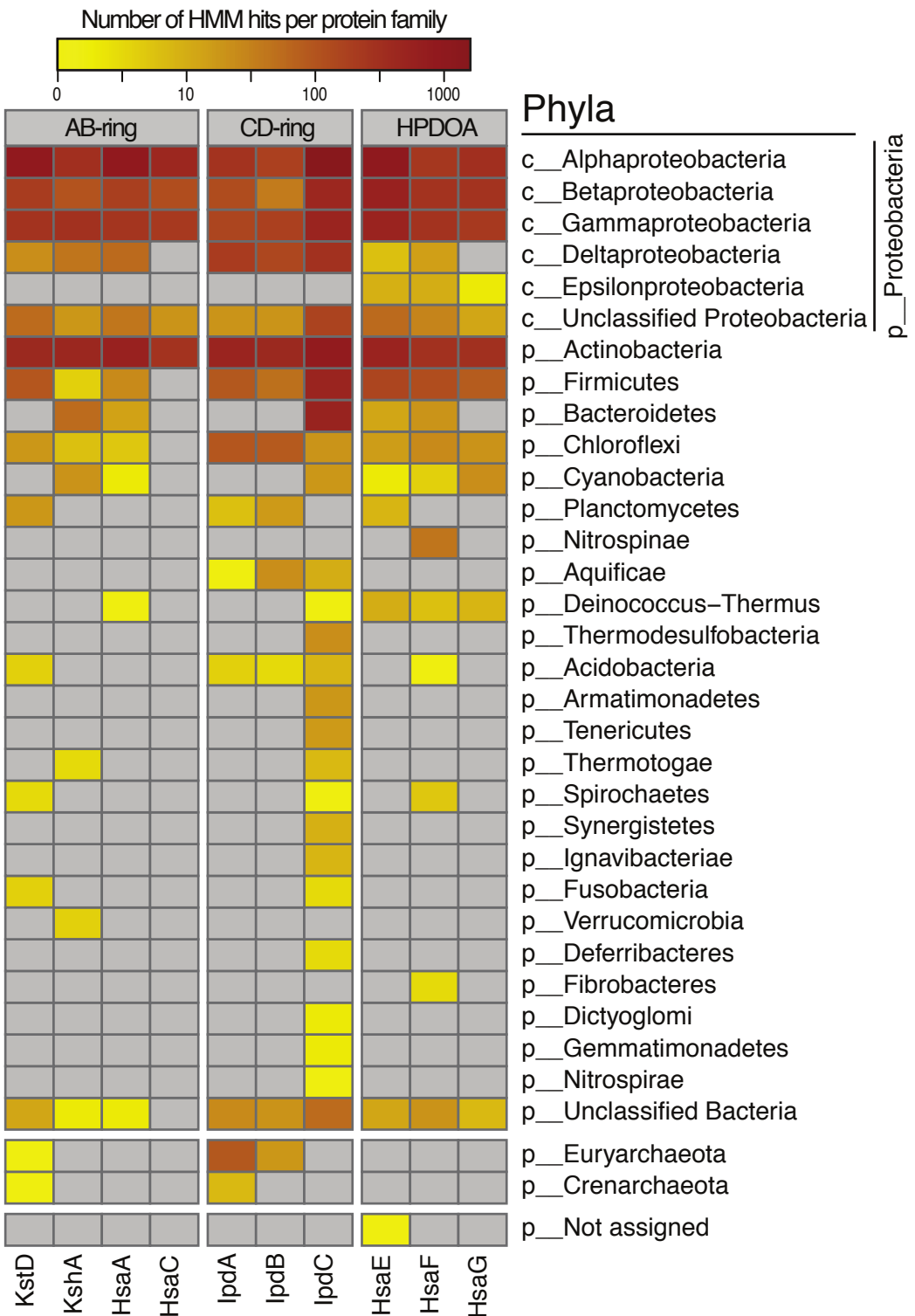
Fig. S2: Number of HMM hits assigned to bacterial and archaeal phyla for each of ten steroid-degradation protein families analyzed.
