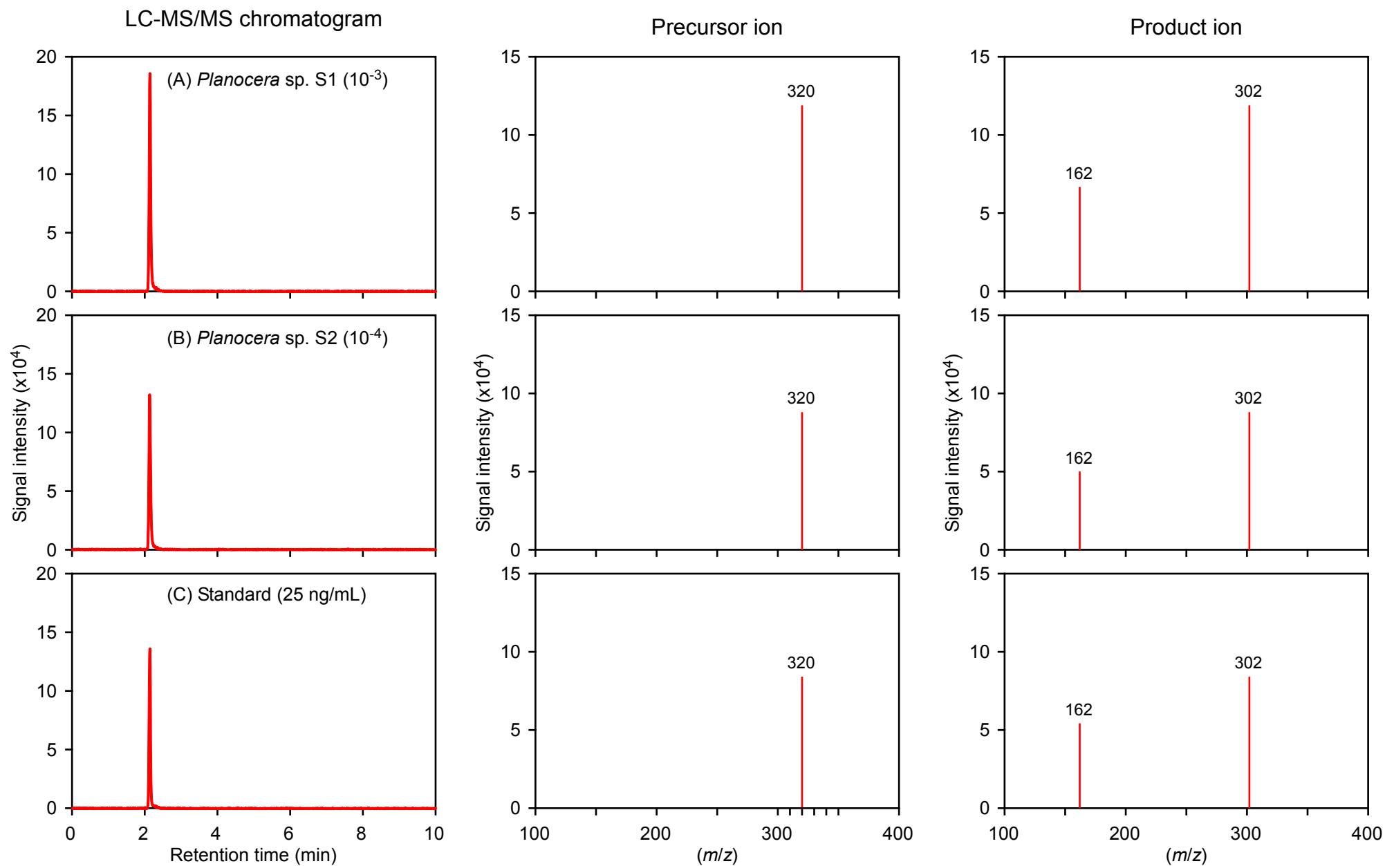
Figure S1. LC-MS/MS patterns of the TTX from planocerid flatworms specimen S1 (A) and S2 (B), and 25 ng/mL TTX standard (C). Left panels represent LC-MS/MS chromatograms, while the middle and right panels represent the mass spectrum of the precursor and product ions, respectively.
