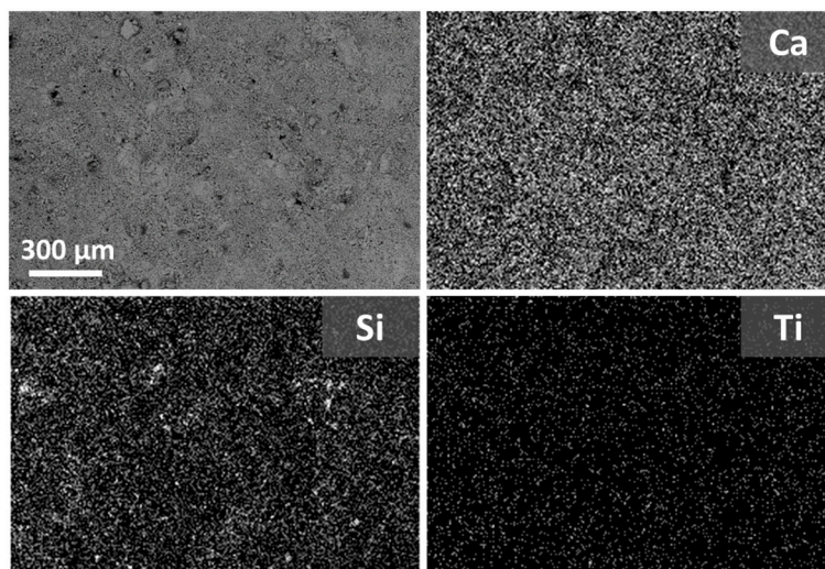
Figure S2. ESEM-EDX images of Ajarte limestone treated with WNC and Ca, Si and Ti maps of distribution.
