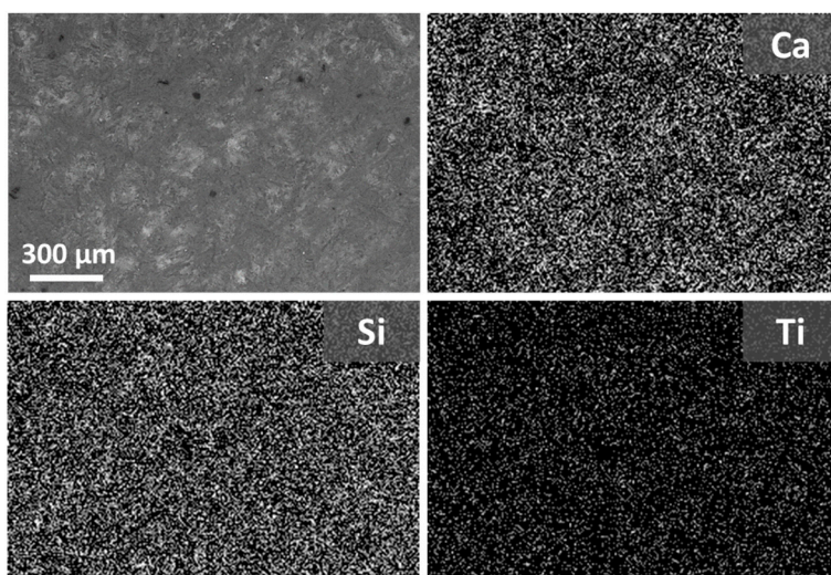
Figure S1. ESEM-EDX images of Apuan marble treated with WNC and Ca, Si and Ti maps of distribution.
