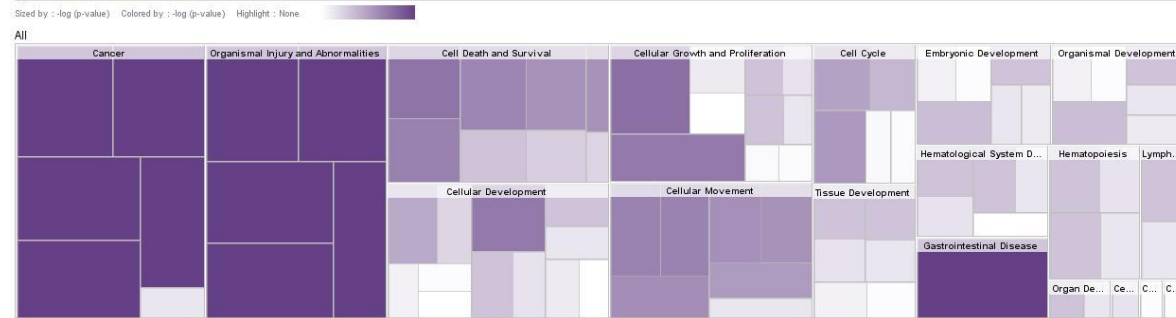
hyb2/MDA - Diseases & Functions
