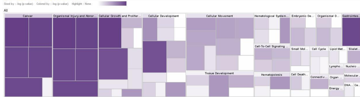
hyb1/MDA - Diseases & Functions
