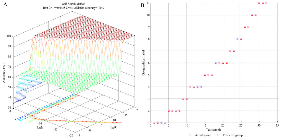
Figure S6: Score plots of the GS-SVM model of mushroom stipe
