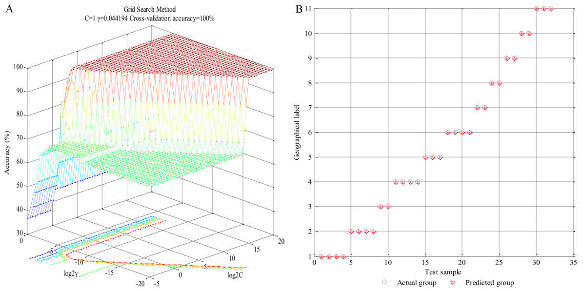
Figure S5: Score plots of the GS-SVM model of mushroom cap
