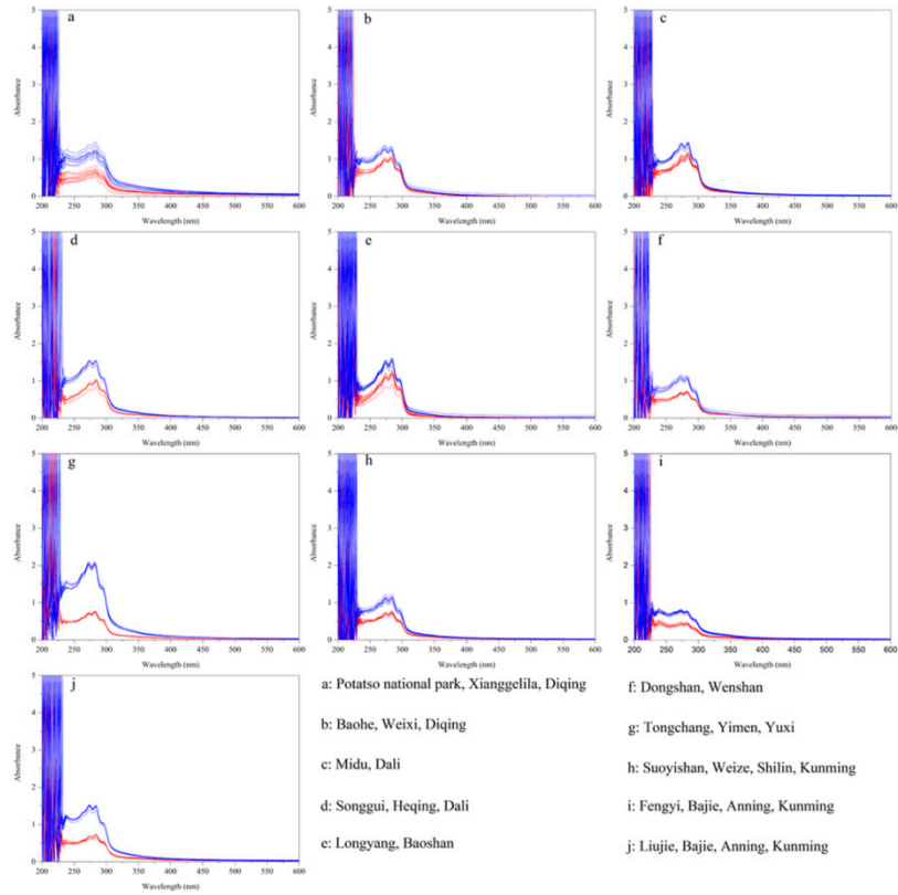
Figure S3: The UV-Vis fingerprints of mushroom chloroform extract from other ten geographical origins
