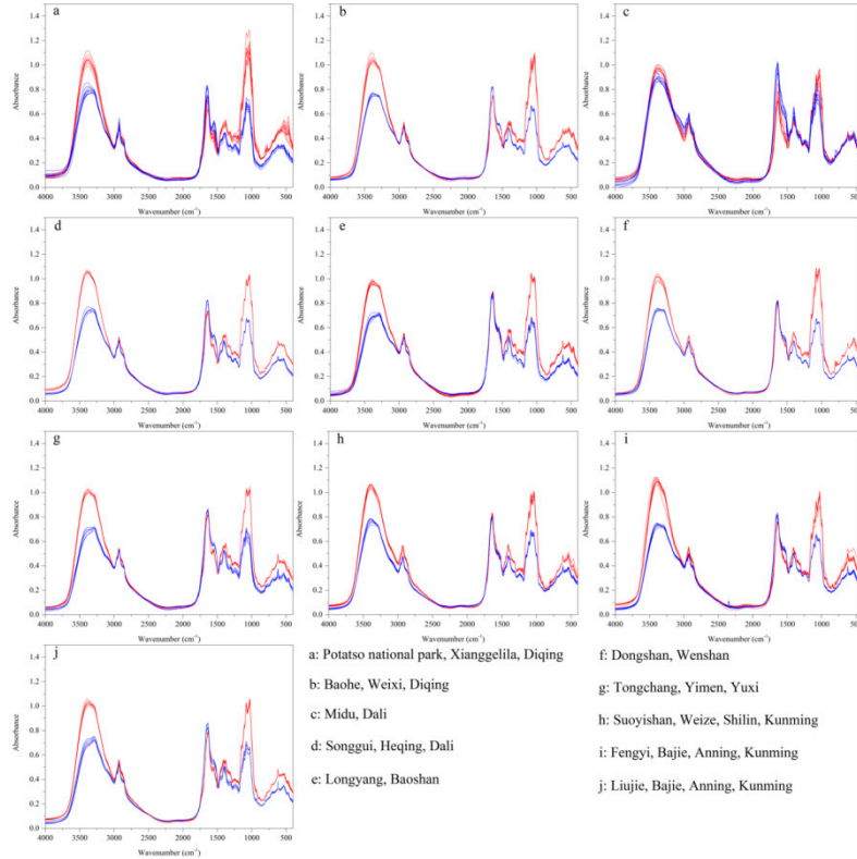
Figure S4: The FT-MIR fingerprints of the mushroom samples from other ten geographical origins
