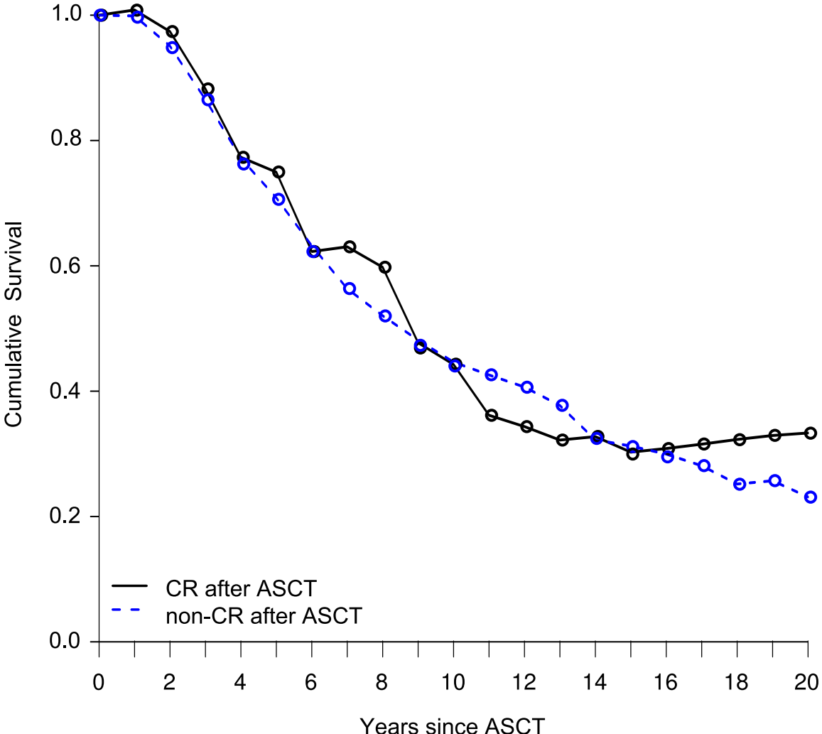
Relative Survival by Response after ASCT
