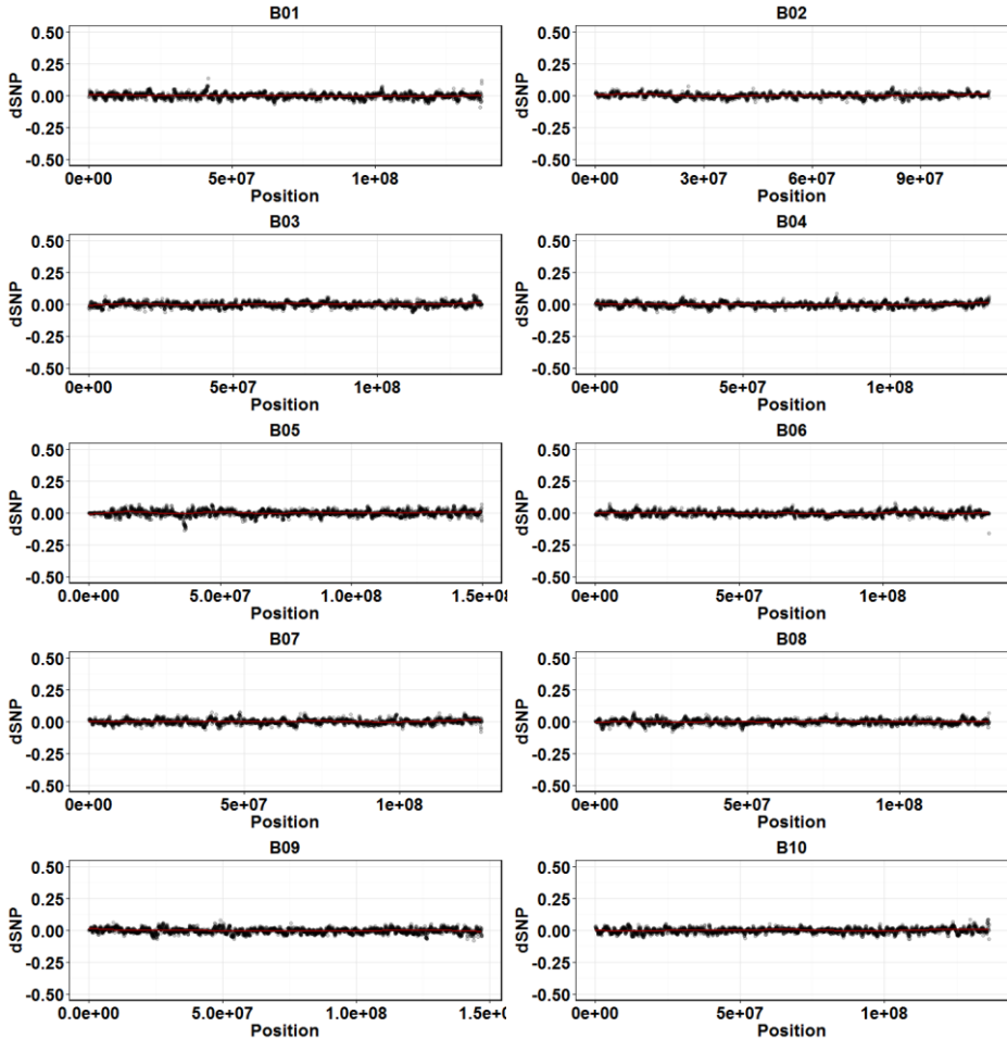
Figure S1 – False positive SNP calls generate noise in analysis. \Delta SNP values were generated using all potential SNPs identified in bulks without knowledge of robust parental SNPs. A sliding window of size 2Mb sliding 500kb was used to calculate a sliding average as a smoothing function and plotted for each chromosome. The false positive SNP calls create so much noise that significant regions cannot
