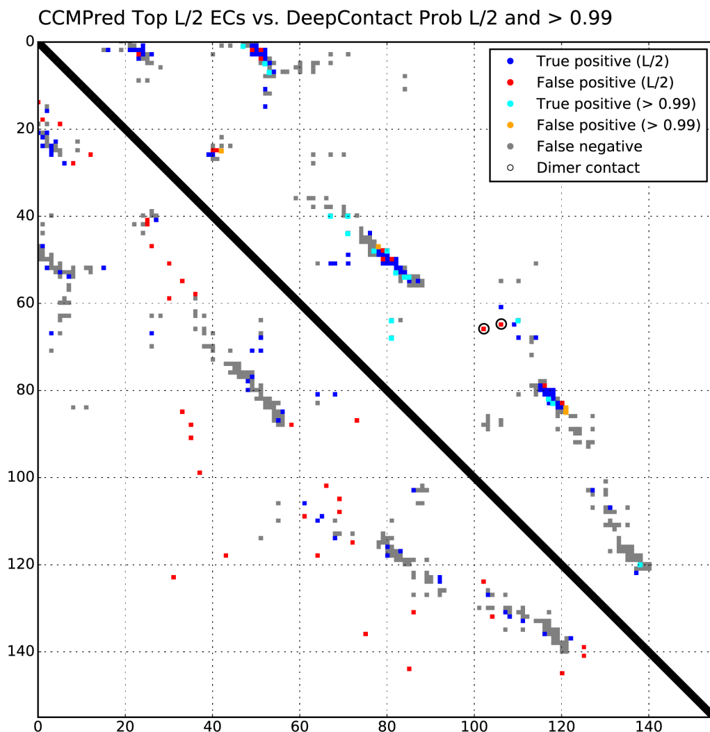
Figure S1. DeepContact integrates local information to improve contact prediction. Related to Figure 3A.
