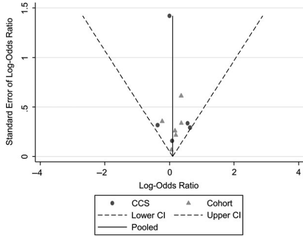
Supplementary Figure S1 Funnel plot, with study variance (i.e. SE of the log-odds ratio, vertical axis) plotted against measure of association (i.e. log-odds ratio, horizontal axis).
