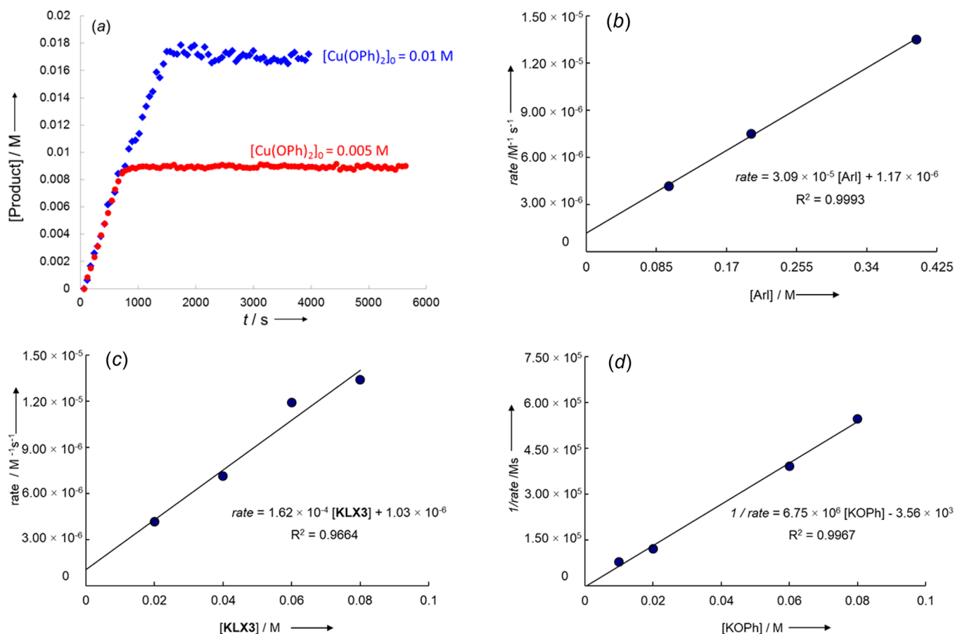
Figure 5. (a) Plot of the rise of the biaryl ether product 2 from the reactions of p -iodotoluene (0.10 M) with 0.010 M (blue diamonds) or 0.005 M (red circles) of \text{KCu}(\text{OPh})_2 ( 1a ) in the presence of \text{KLX3} (0.080 M) in \text{DMSO}-d_6 at 50 °C. (b) Plot of the [p\text{-iodotoluene}] vs the initial rate for the rise of the biaryl ether product 4 from the reaction of p -iodotoluene (0.10–0.40 M) with \text{KCu}(\text{OPh})_2 ( 1a , 0.01 M) in the presence of \text{KLX3} (0.02 M) in \text{DMSO}-d_6 at 50 °C. (c) Plot of the concentration of the ligand \text{KLX3} ( [\text{L}] , 0.02–0.08 M) vs the initial rate for the rise of the biaryl ether product 2 from the reaction of p -iodotoluene (0.10 M) with \text{KCu}(\text{OPh})_2 ( 1a , 0.01 M) in \text{DMSO}-d_6 at 50 °C. (d) Plot of the added [\text{KOPh}] (0.010–0.080 M) vs the reciprocal of the initial rate ( 1/\text{rate} ) for the rise of the biaryl ether product 4 from the reaction of p -iodotoluene (0.20 M) with \text{KCu}(\text{OPh})_2 ( 1a , 0.01 M) in the presence of \text{KLX3} (0.02 M) in \text{DMSO}-d_6 at 50 °C.
