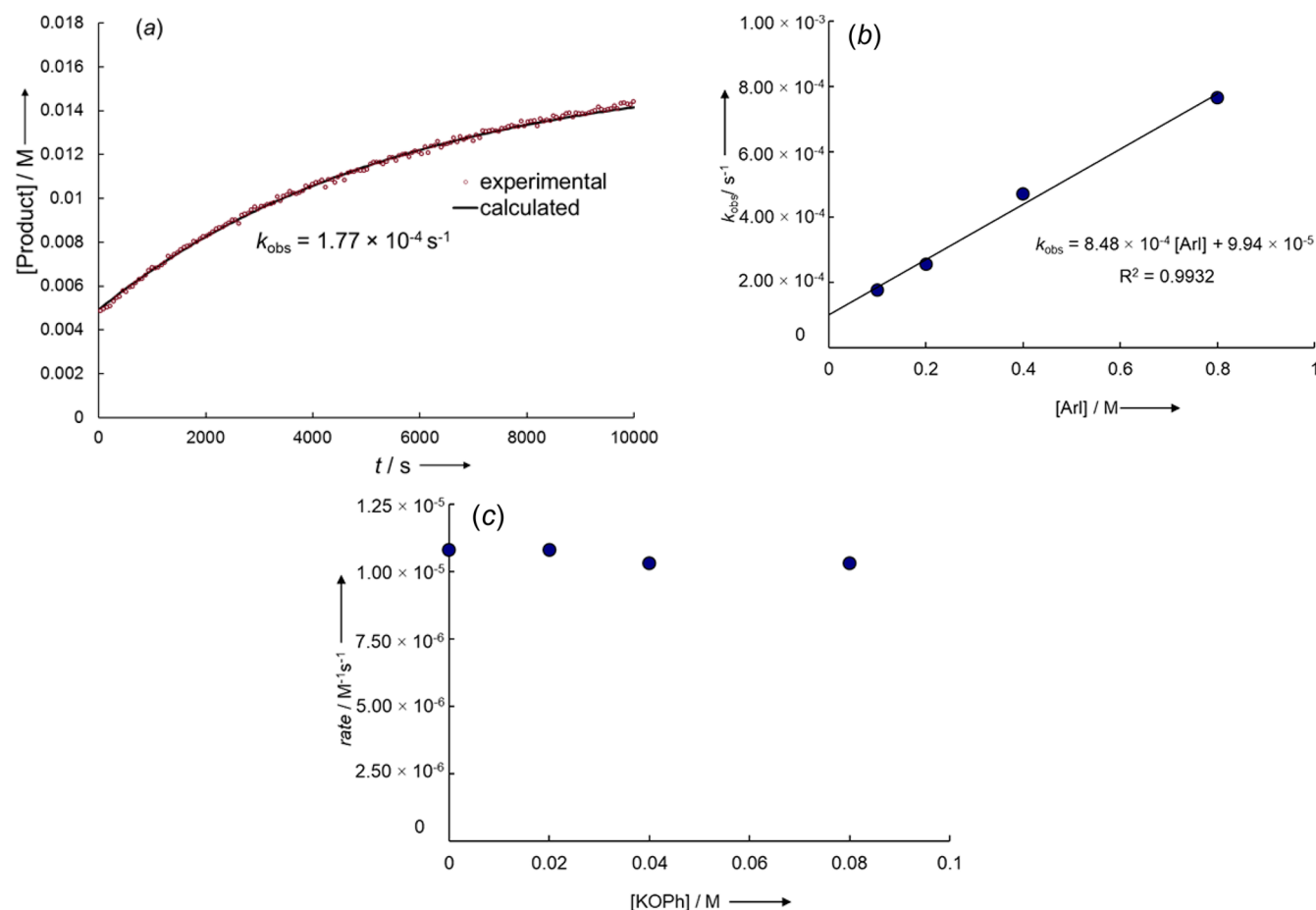
Figure 4. (a) Plot of the formation of the product 2 from the reaction of p -iodotoluene (0.20 M) with \text{K}[\text{Cu}(\text{LX1})\text{OPh}] generated in situ from the reaction of KLX1 (0.010 M) with \text{KCu}(\text{OPh})_2 ( 1a ) (0.010 M) in \text{DMSO}-d_6 at 30 °C. (b) Plot of k_{\text{obs}} versus [ p -iodotoluene] for the reaction of p -iodotoluene (0.10–0.80 M) with \text{K}[\text{Cu}(\text{LX1})\text{OPh}] generated in situ from the reaction of KLX1 (0.010 M) with \text{KCu}(\text{OPh})_2 ( 1a ) (0.010 M) in \text{DMSO}-d_6 at 30 °C. (c) Plot of the added [\text{KOPh}] (0.00–0.080 M) vs the initial rate for the formation of the product 2 from the reaction of p -iodotoluene (0.10 M) with \text{K}[\text{Cu}(\text{LX1})\text{OPh}] generated in situ from the reaction of KLX1 (0.010 M) with \text{KCu}(\text{OPh})_2 ( 1a ) (0.010 M) in \text{DMSO}-d_6 at 50 °C.
