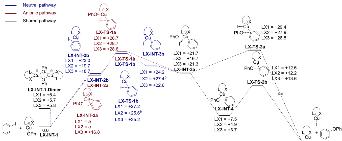
Figure 9. Computed reaction pathways for Ullmann etherification of aryl iodides in the presence of anionic ligands LX (the numbers correspond to computed values of \Delta G/\text{kcal}\cdot\text{mol}^{-1} ). a All attempts to optimize the geometry of this structure were unsuccessful. b LX-INT-3b is 2.5 kcal/mol downhill to LX-TS-1b in gas phase.
