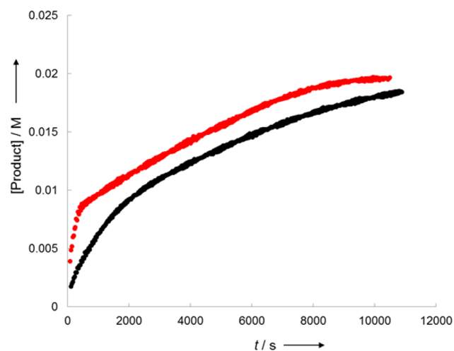
Figure 6. Reaction of 1a (10 mM) with 4-iodotoluene (100 mM) in the presence of \text{KLX3} (80 mM) in the absence of \text{CuI} (black) or presence of \text{CuI} (10 mM, red line) in \text{DMSO} at 30 °C.
