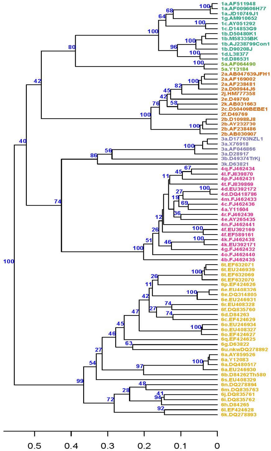
UPGMA Tree RefSeqs v070113 (K80, gamma=0.42)
