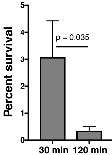
Figure S2. Long periods of incubation with gentamicin post-phagocytosis can affect S. gordonii survival.
