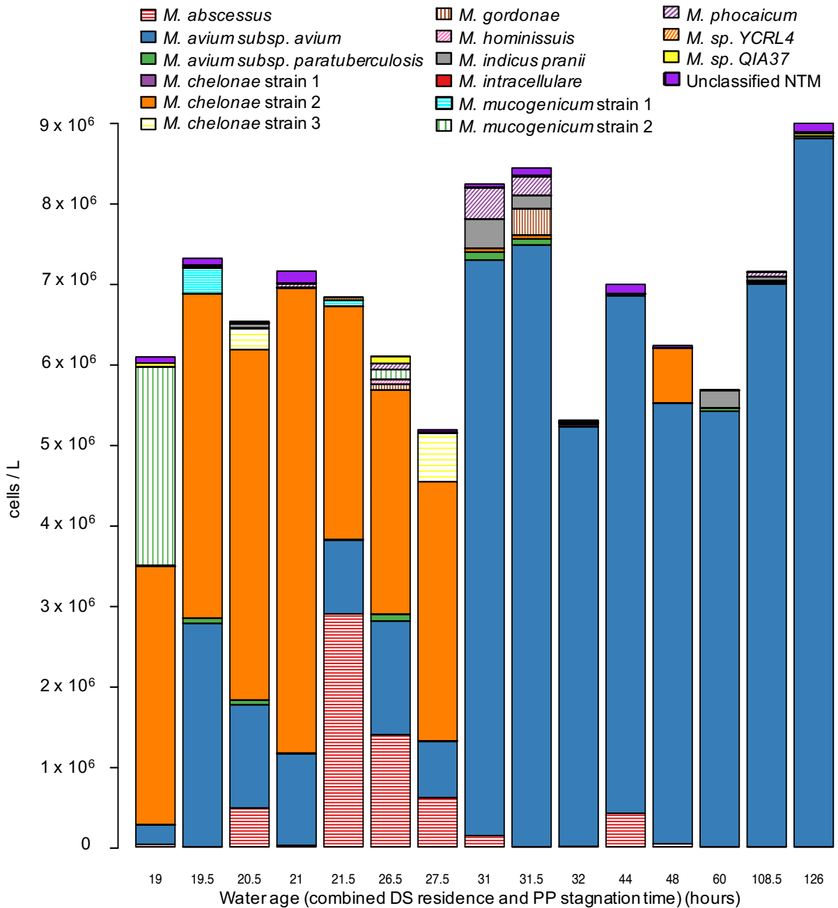
SI-4. Concentration (cells/L) of NTM species and strains in biomass from 15 drinking water samples collected from premise plumbing. The concentrations were calculated by combining qPCR and PacBio data. Water age represents the total of water residence time in the distribution system and stagnation time in premise plumbing.
