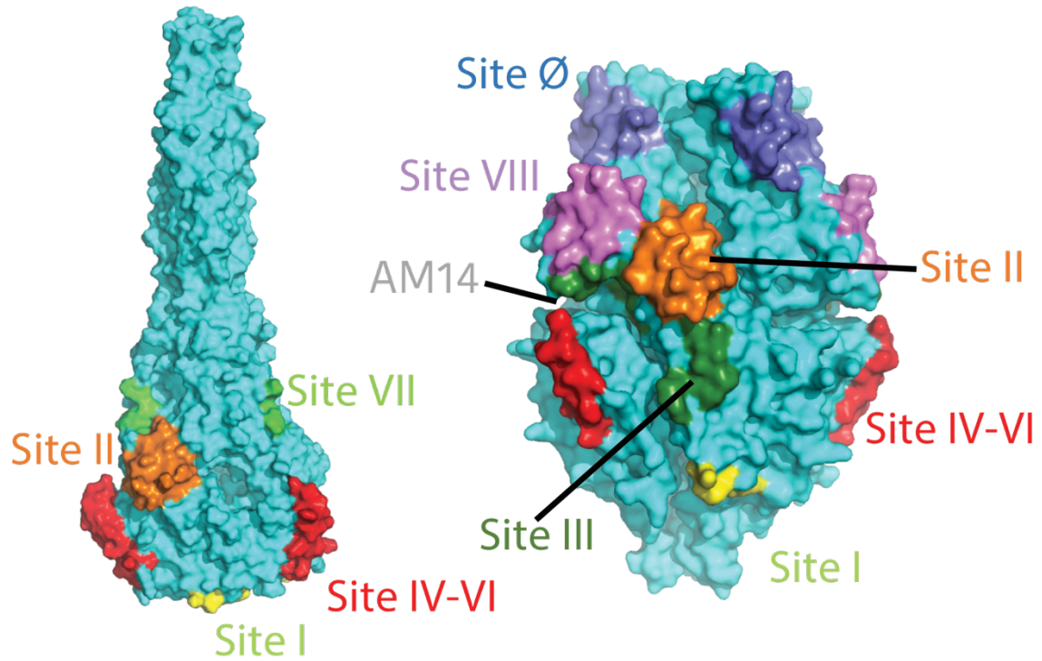
Fig. S1. Summary of known antigenic sites on the RSV F protein.
