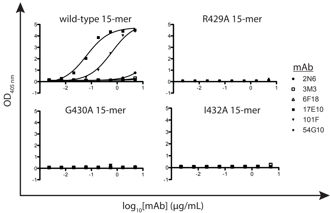
Fig. S7. ELISA binding curves of site IV mAbs to biotinylated site IV 15-mer peptides coated on streptavidin ELISA plates. Data points are the average of two technical replicates. Error bars indicate the range of the two measurements.
