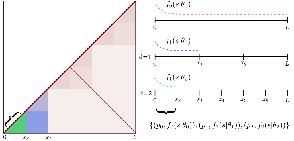
Figure 4. Approximating the structurally related modulation of observed contact frequencies. Beyond primary intra-chromosomal interactions which produce the main diagonal, Sim3C can reproduce an inter-arm mediated anti-diagonal at user controlled intensity. Illustrated here, finer scale modulations attributed to topologically associated domains (TADs) can optionally be approximated. Primary interactions are governed by the empirical distribution f_0(s|0) which covers the full interval [0, L) . Each level of recursion ( d = 1, 2 \dots n ) generates a finer set of intervals, to which a distribution f_i(s|\theta_i) and probability p_i is assigned. The intervals at the final depth each define a range (green, curly braces) over which a set of probabilities and empirical distribution pairs govern interaction separation s .
