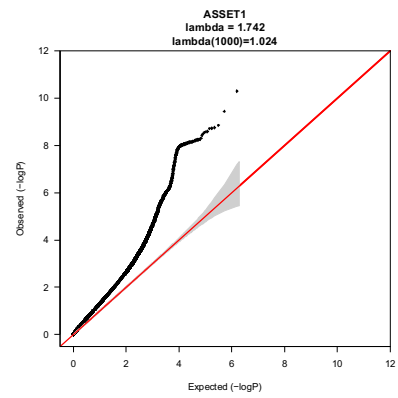
Figure S14. QQ Plots
