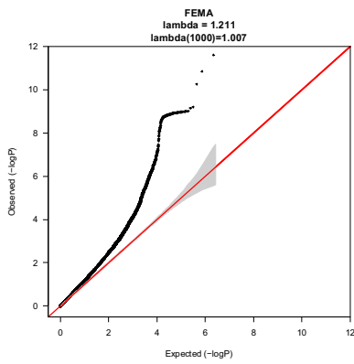
Figure S14. QQ Plots
