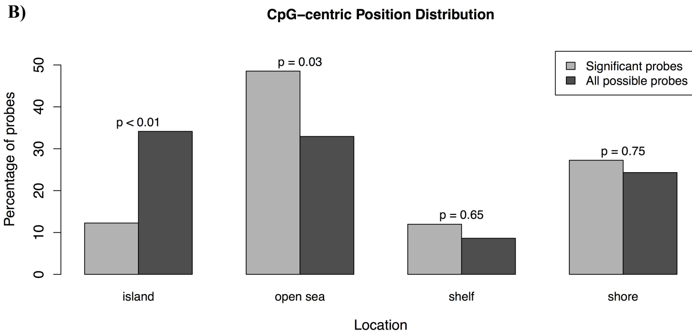
Supplementary Figure 2. Distribution of significantly differentially methylated positions in transcriptional cluster 2 (versus transcriptional cluster 1, corrected for fetal sex and gestational age) (light grey) compared to the full set of possible methylation probes (dark grey), in terms of their (A) gene region locations and (B) CpG region locations. P-values were obtained from Fisher's exact tests.
