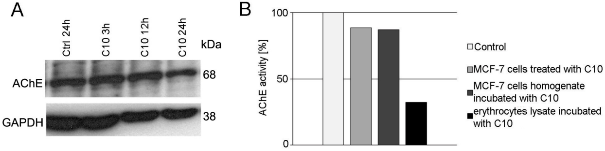
Supplemental Figure 2. AChE protein level and activity in MCF-7 cells after C10 treatment. (A) Representative western blot of AChE protein level in control MCF-7 cells and treated with C10 for the indicated time. (B) AChE activity in MCF-7 cells, homogenate of these cells or erythrocyte lysate treated with IC50 dose of C10. Graph represents mean value from 2 independent experiments.
