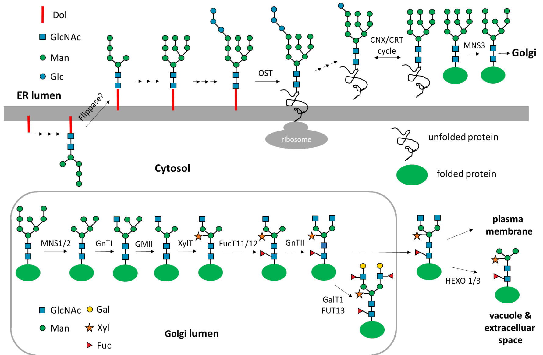
Figure S1. Schematic diagram outlining the N -glycan biosynthesis pathway in ER and Golgi apparatus of plants. The red arrow indicates where we could refine the N -glycan biosynthetic model from our data. Dol: dolichol, OST: oligosaccharyltransferase, CNX/CRT cycle: calnexin/calreticulin (CNX/CRT) cycle, MNS: α-mannosidase, GnT: 1,2- N -acetylglucosaminyltransferase, FucT: fucosyltransferase, XylT: xylosyltransferase, GM: α-mannosidase, HEXO: β- N -acetylhexosaminidase, GalT: galactosyltransferase.
