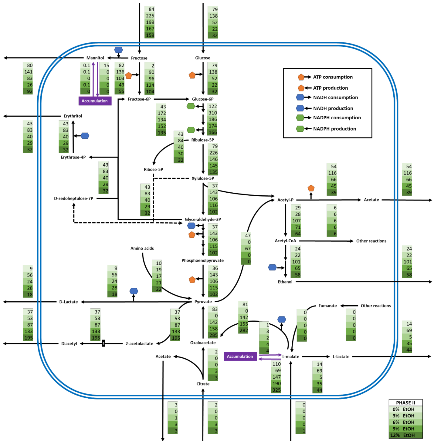
Supplementary Figure S4. Metabolic flux redistribution of the central carbon metabolic pathways of O. oeni PSU-1 upon cultivation in a culture medium without and with 3, 6, 9 and 12% (green boxes, from top to bottom) ethanol concentration, during growth phase II.
