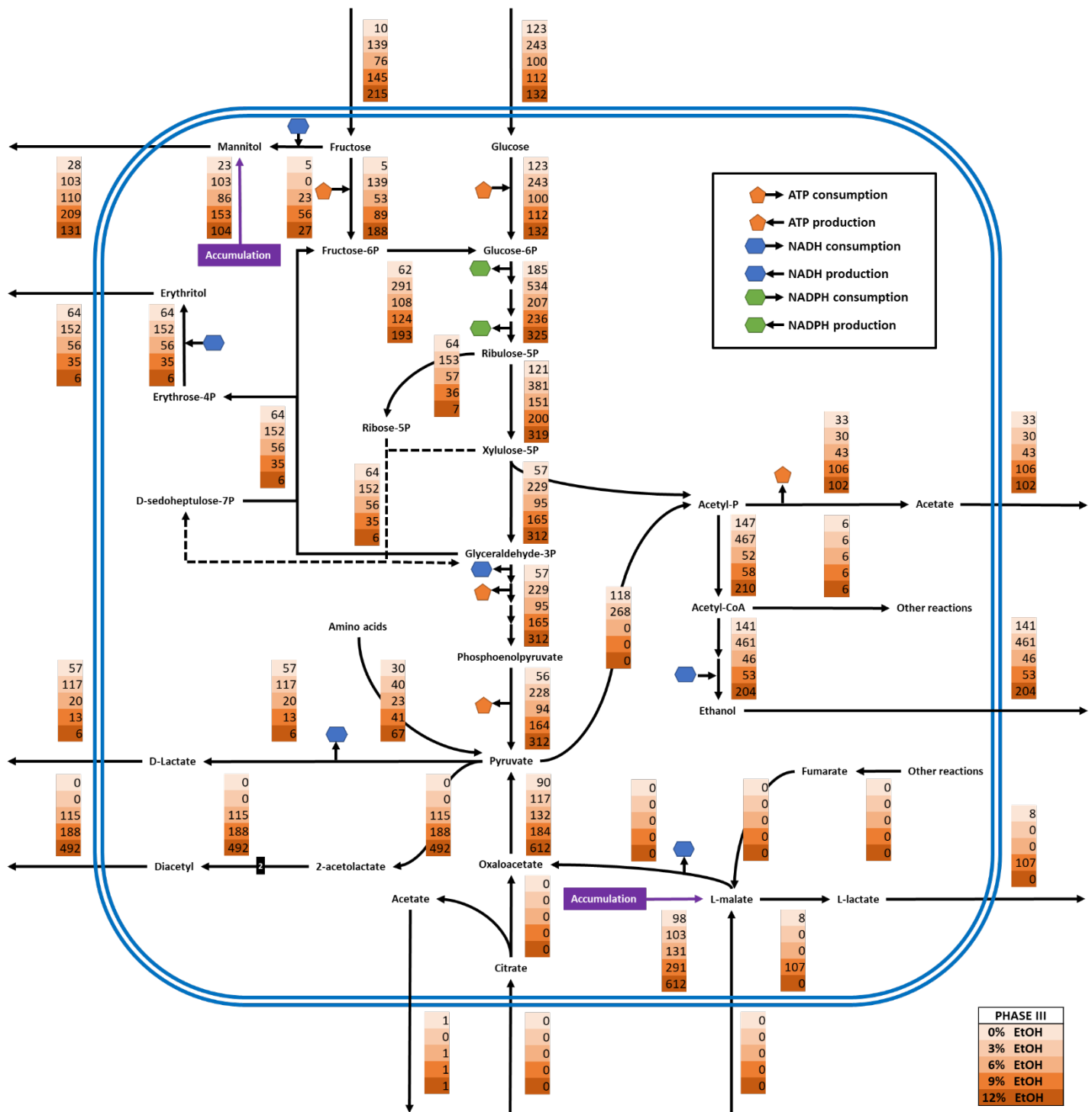
Supplementary Figure S5. Metabolic flux redistribution of the central carbon metabolic pathways of O. oeni PSU-1 upon cultivation in a culture medium without and with 3, 6, 9 and 12% (orange boxes, from top to bottom) ethanol concentration, during growth phase III.
