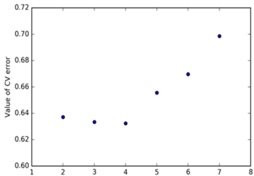
Figure S2 Cross-validation error plot indicating the choice of the appropriate K value.
