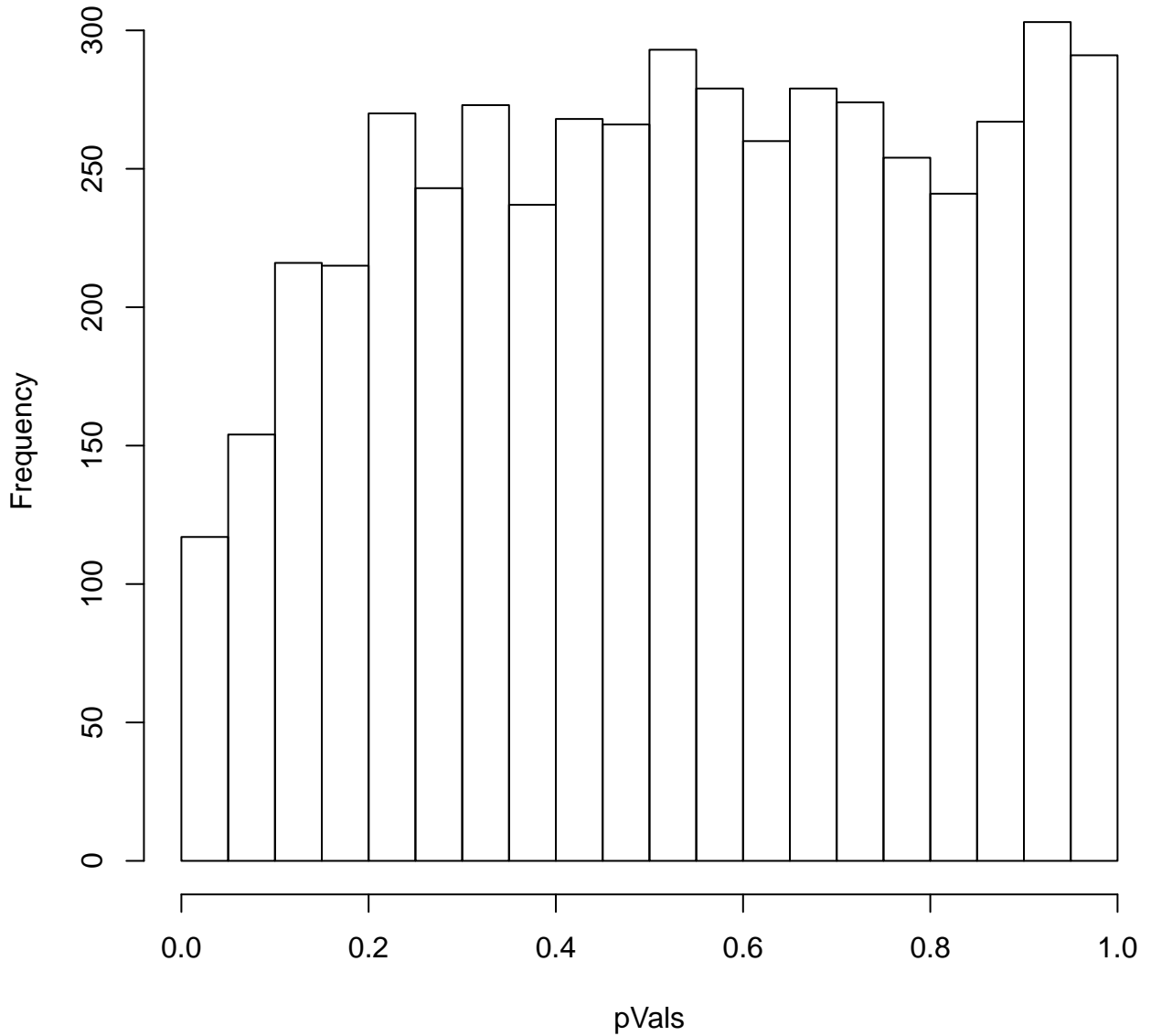
Histogram for pVals for READ
