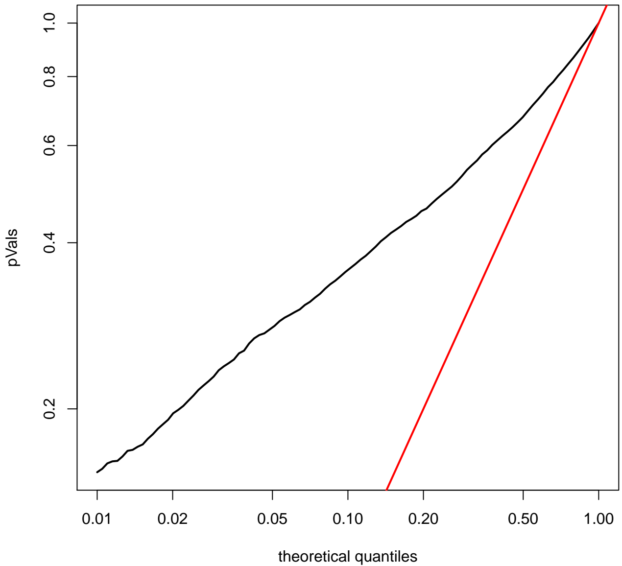
quantile plot for ESCA (log-scale)
