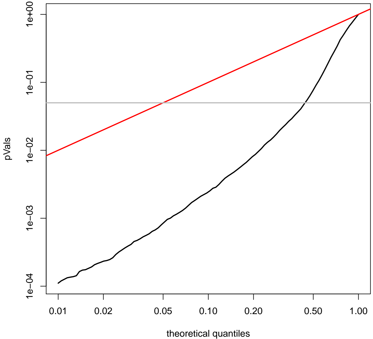
quantile plot for PAAD (log-scale)
