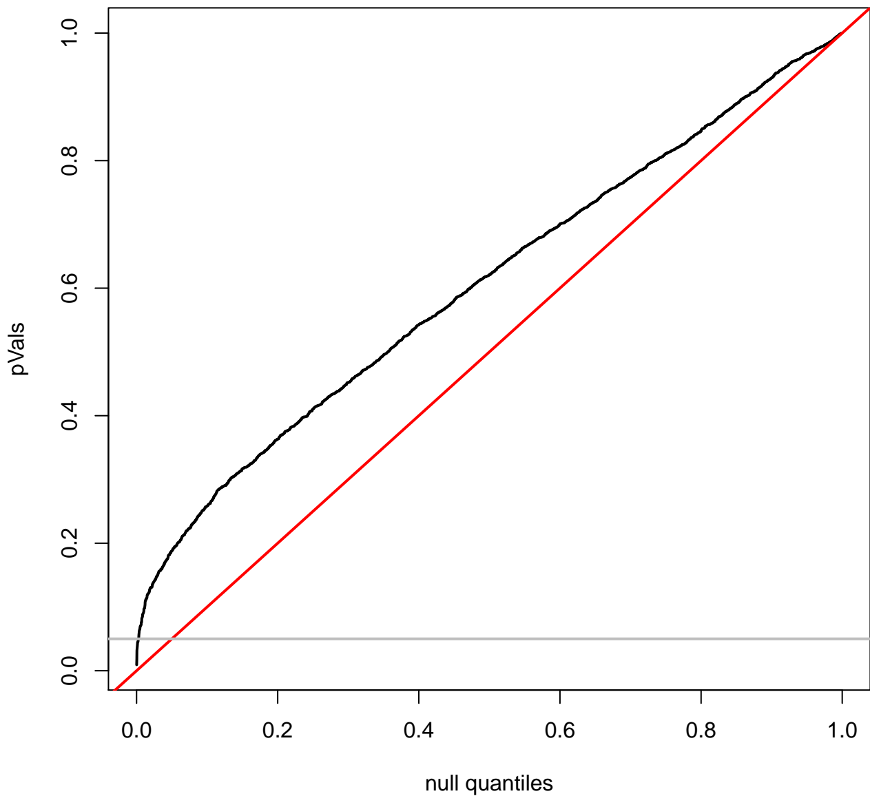
quantile plot for LAML
