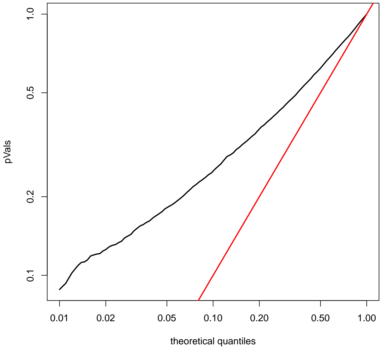
quantile plot for LAML (log-scale)
