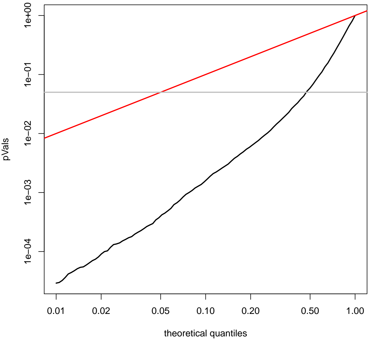
quantile plot for LUAD (log-scale)
