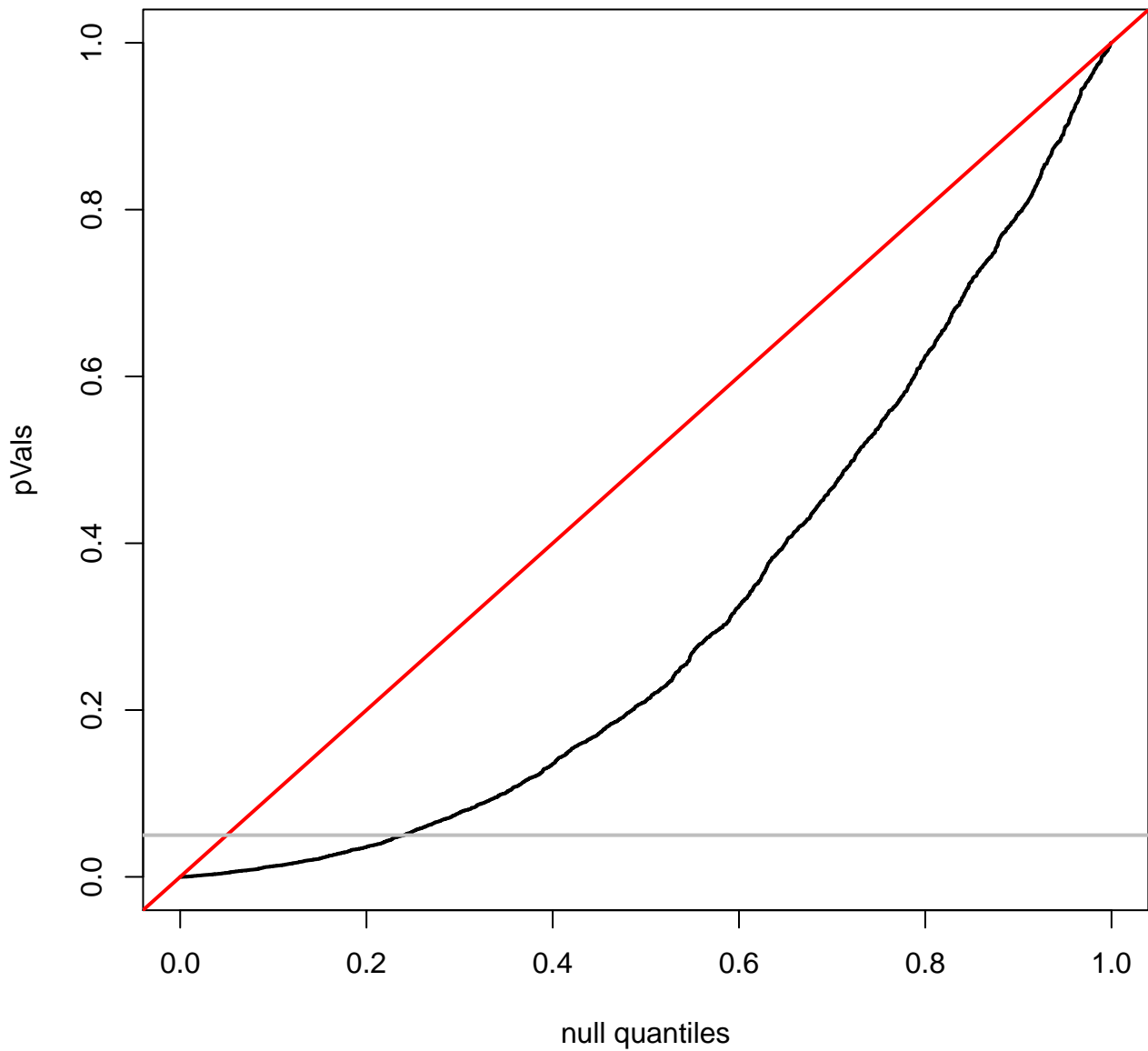
quantile plot for HNSC
