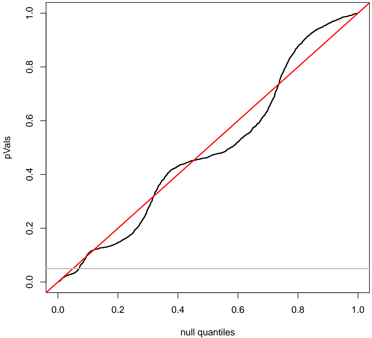
quantile plot for KICH
