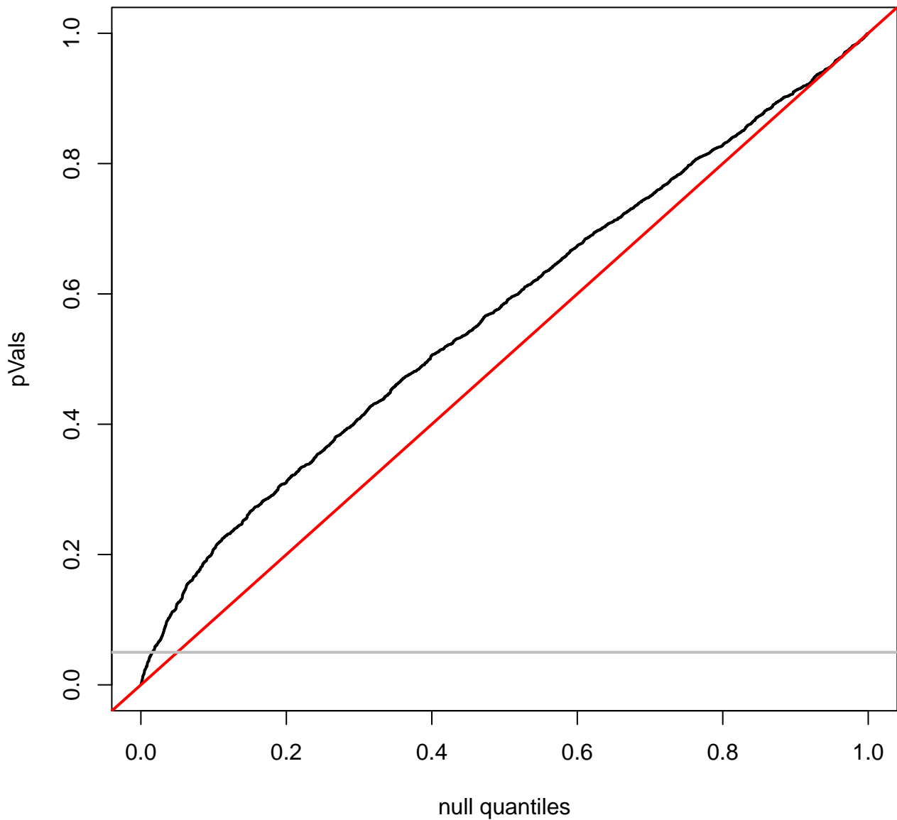
quantile plot for UCS
