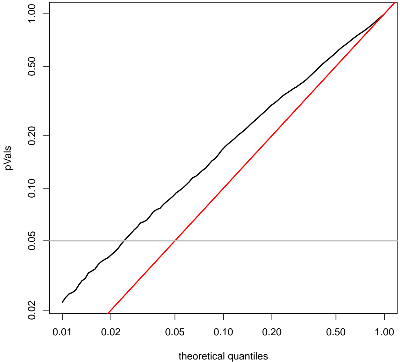
quantile plot for THCA (log-scale)
