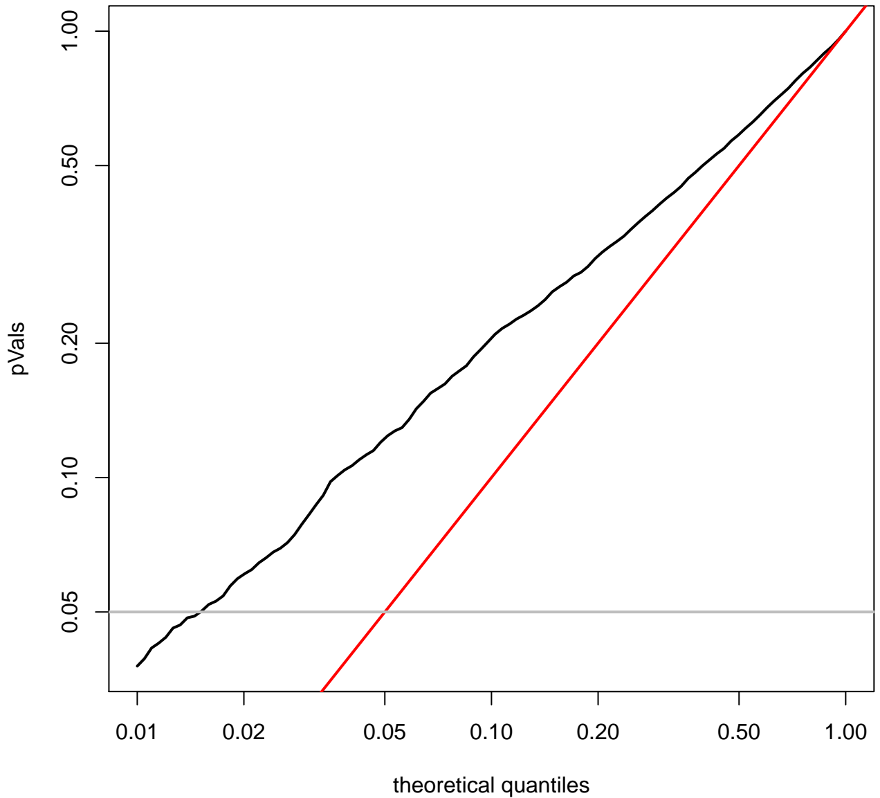
quantile plot for UCS (log-scale)
