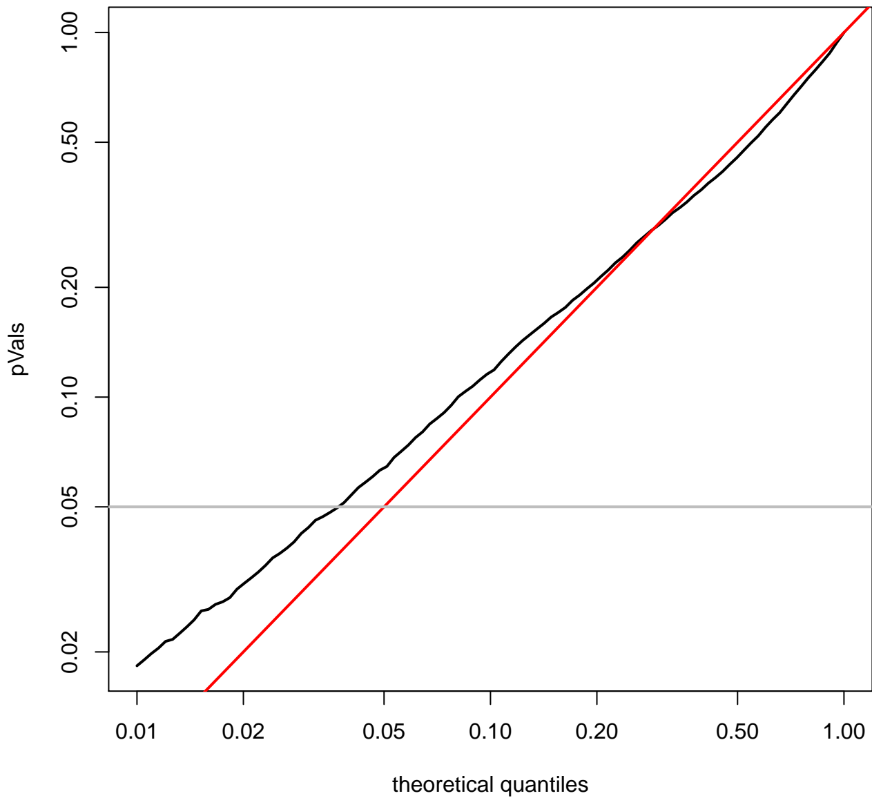
quantile plot for SKCM (log-scale)
