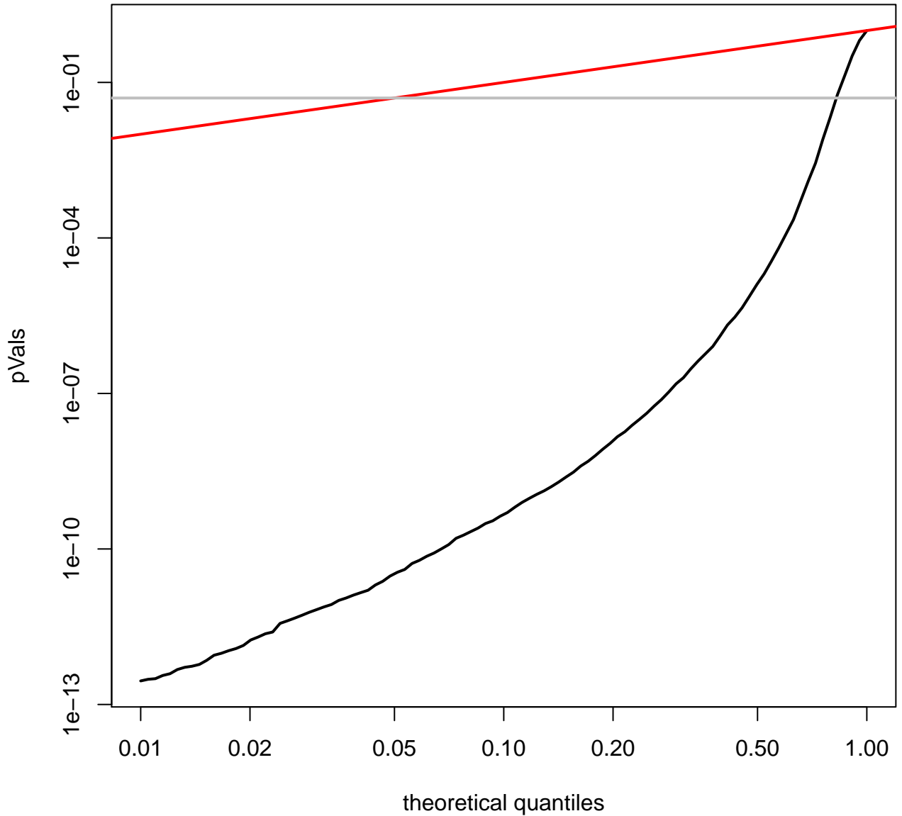
quantile plot for KIRC (log-scale)
