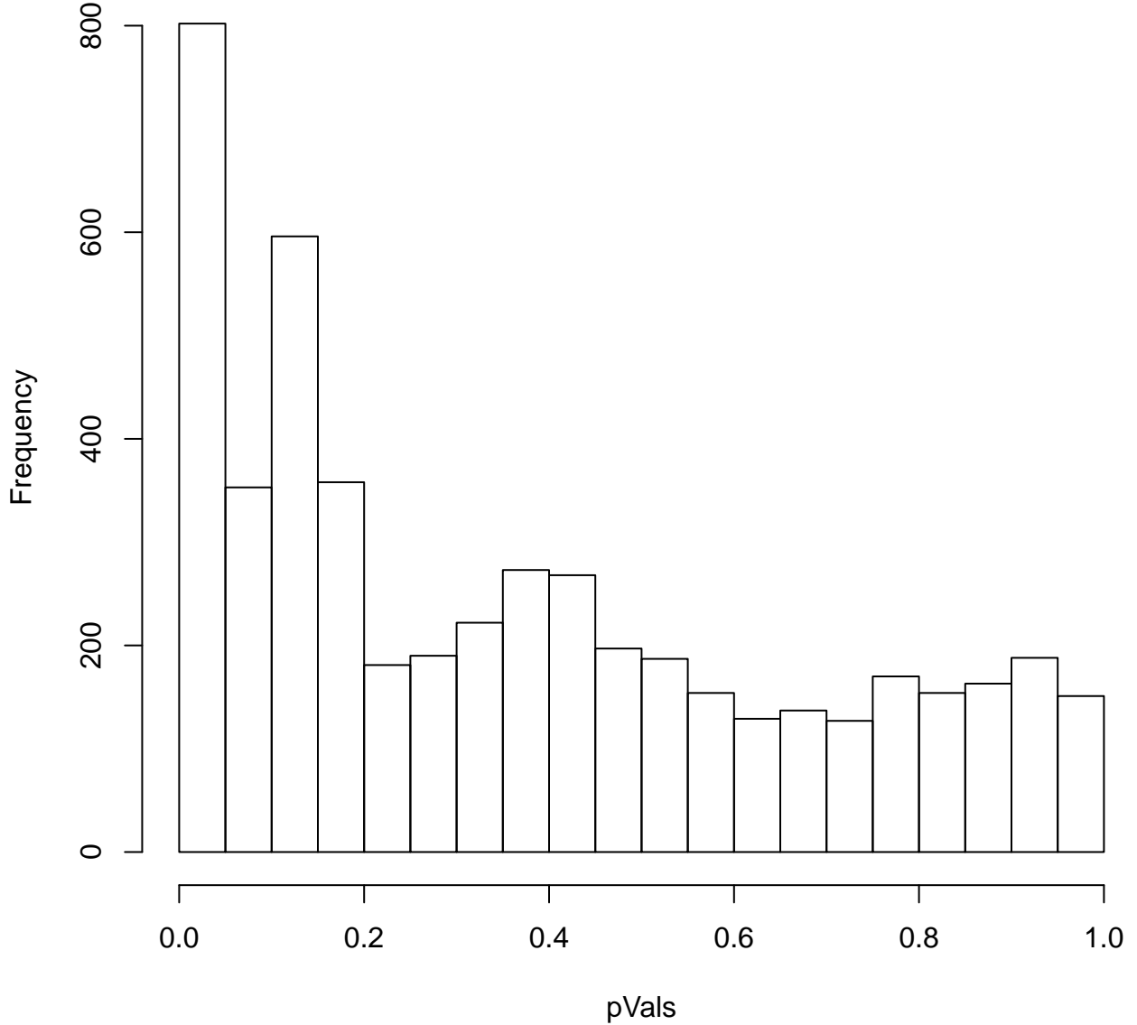
Histogram for pVals for THYM
