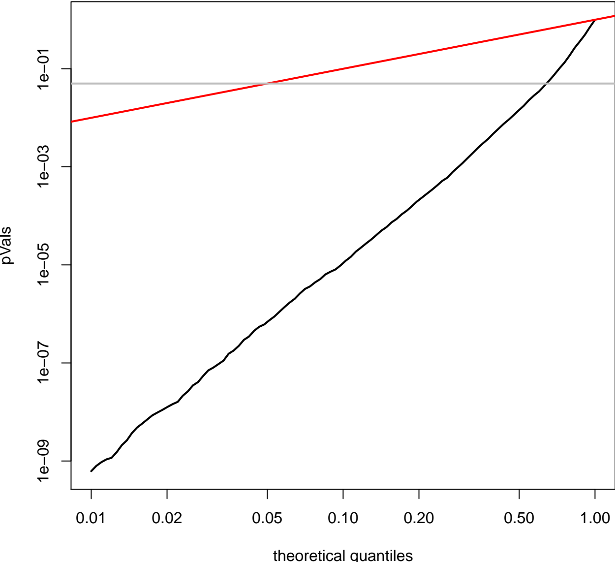
quantile plot for KIPAN (log-scale)
