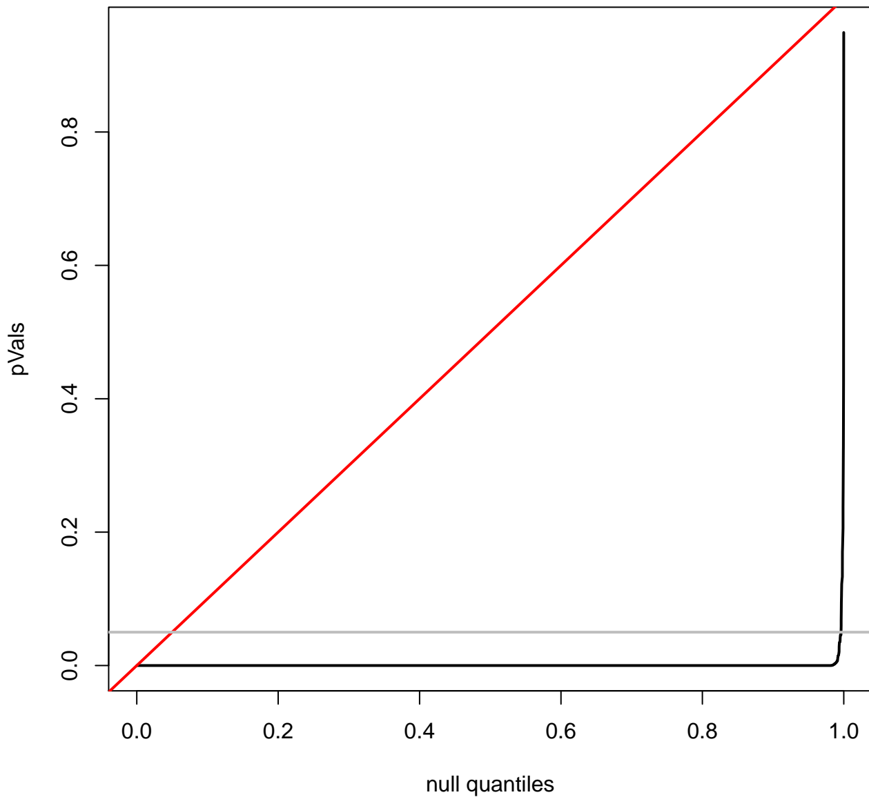
quantile plot for GBMLGG
