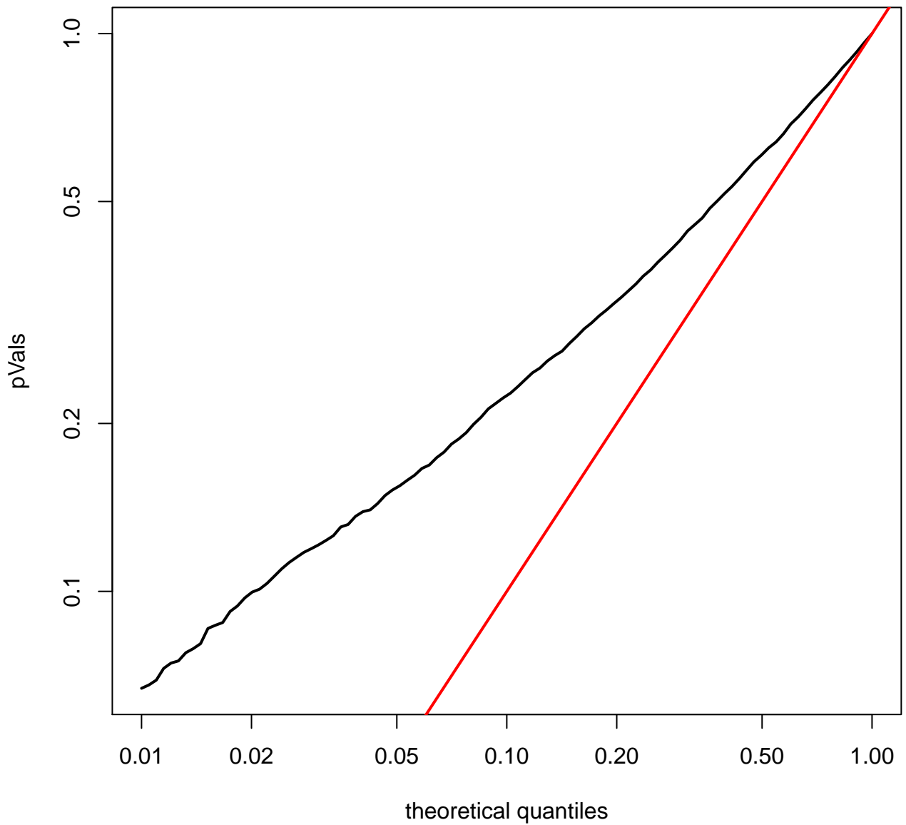
quantile plot for CHOL (log-scale)
