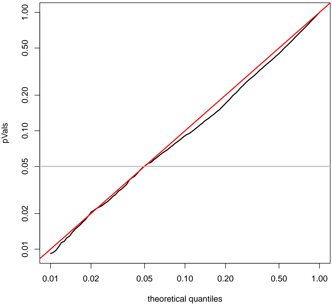
quantile plot for COADREAD (log-scale)
