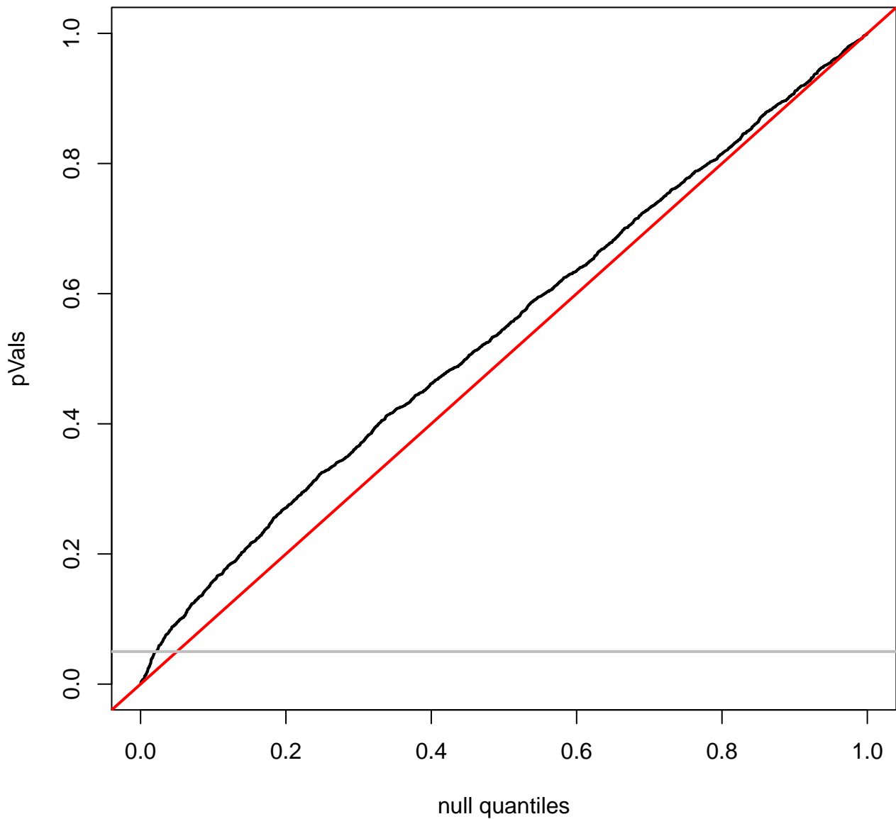
quantile plot for COAD
