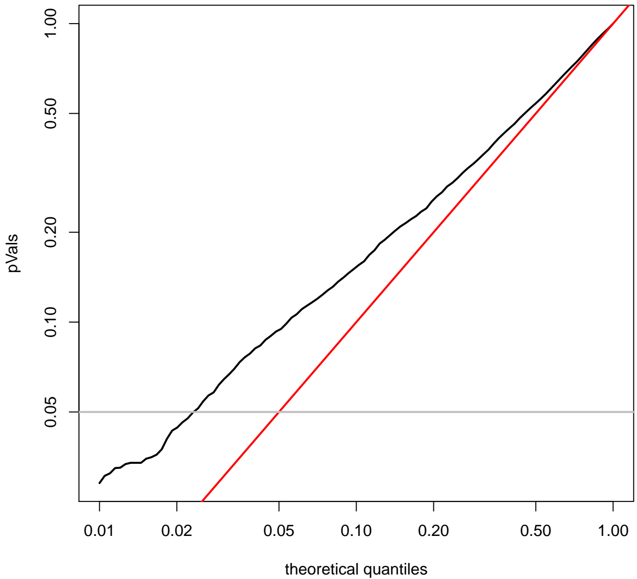
quantile plot for READ (log-scale)
