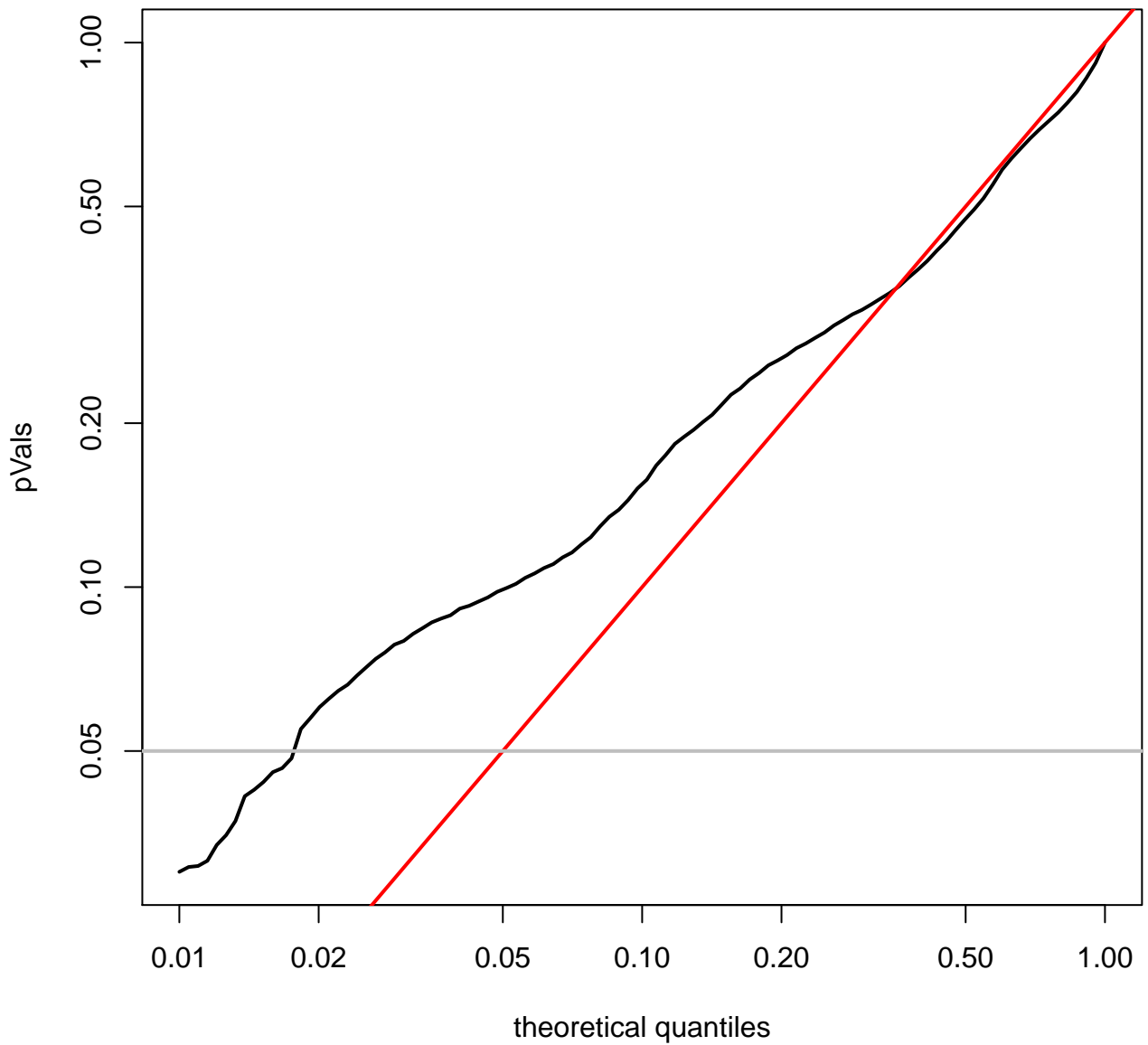
quantile plot for PRAD (log-scale)
