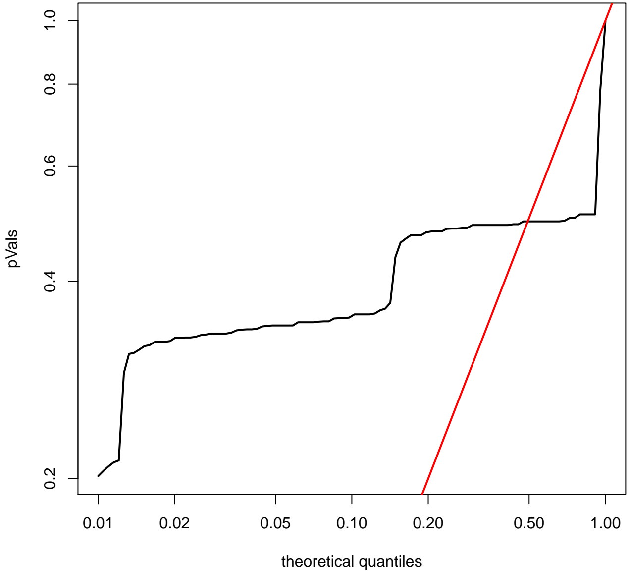
quantile plot for TGCT (log-scale)
