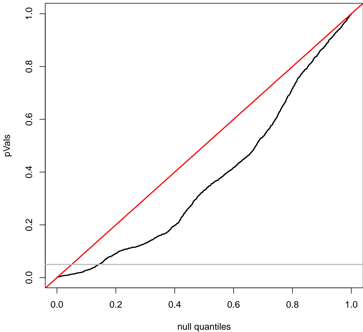
quantile plot for THYM
