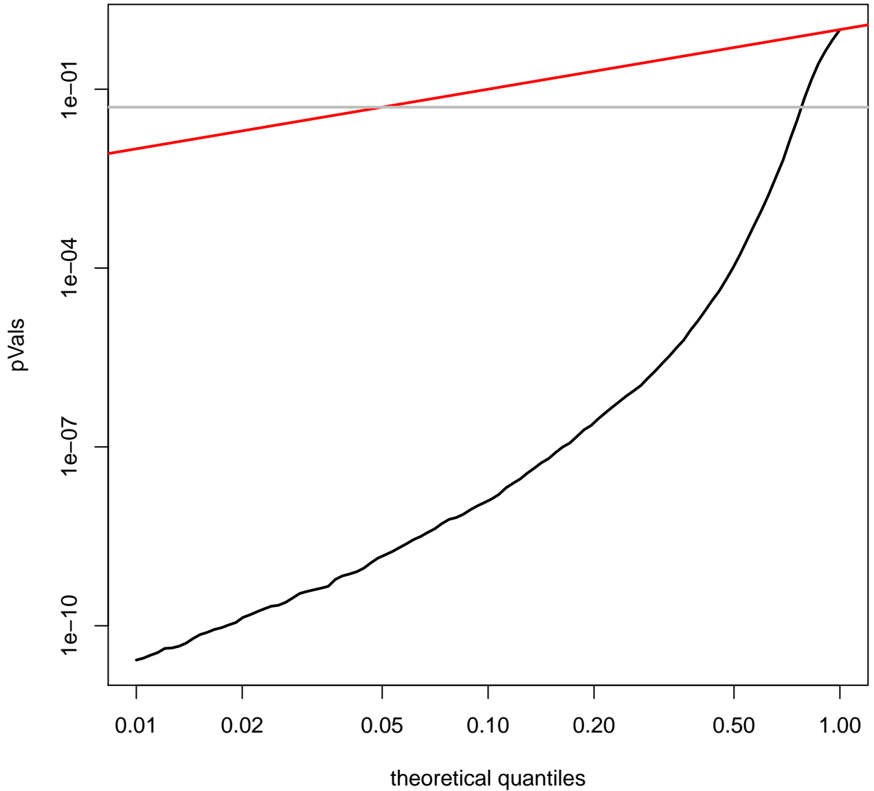
quantile plot for LGG (log-scale)
