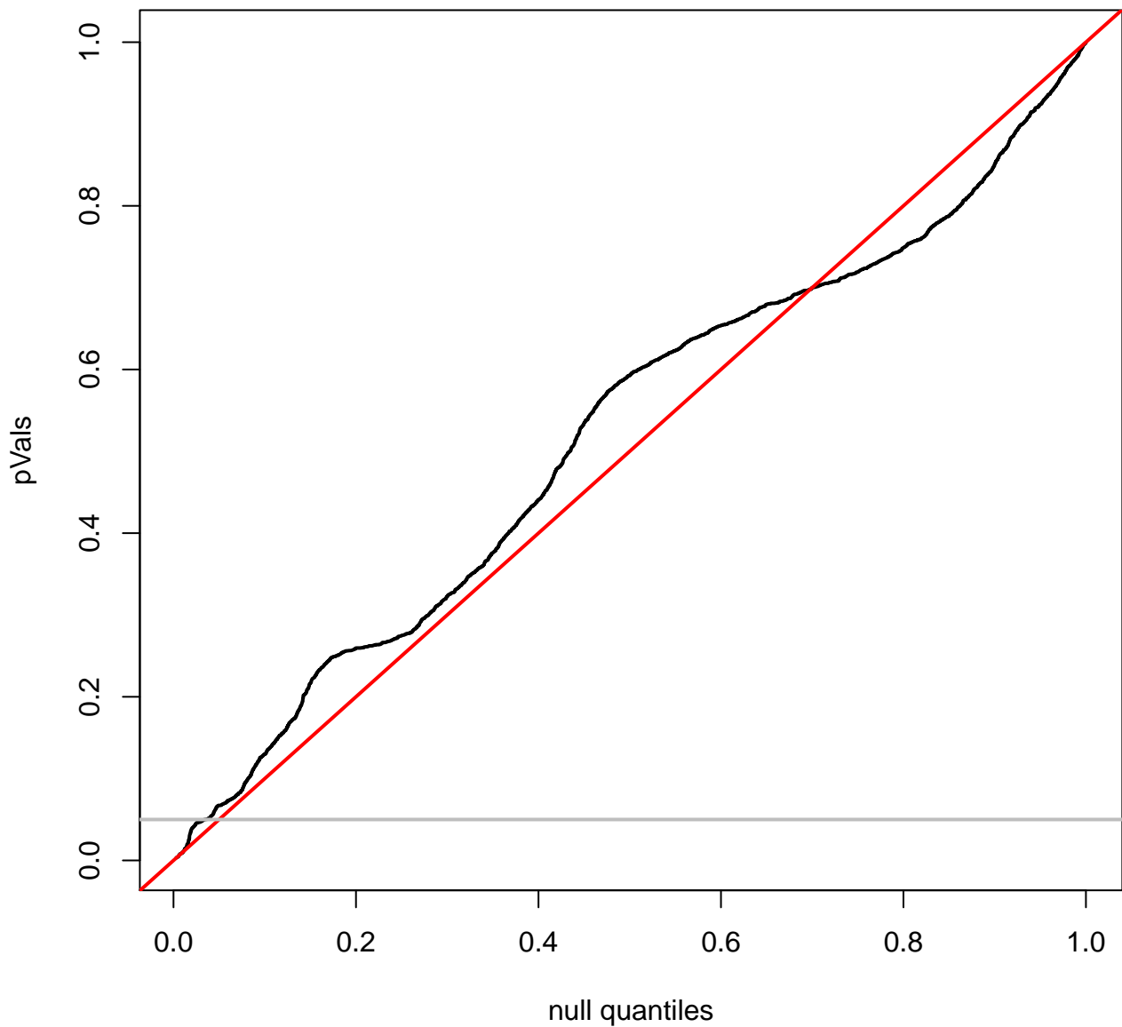
quantile plot for PCPG
