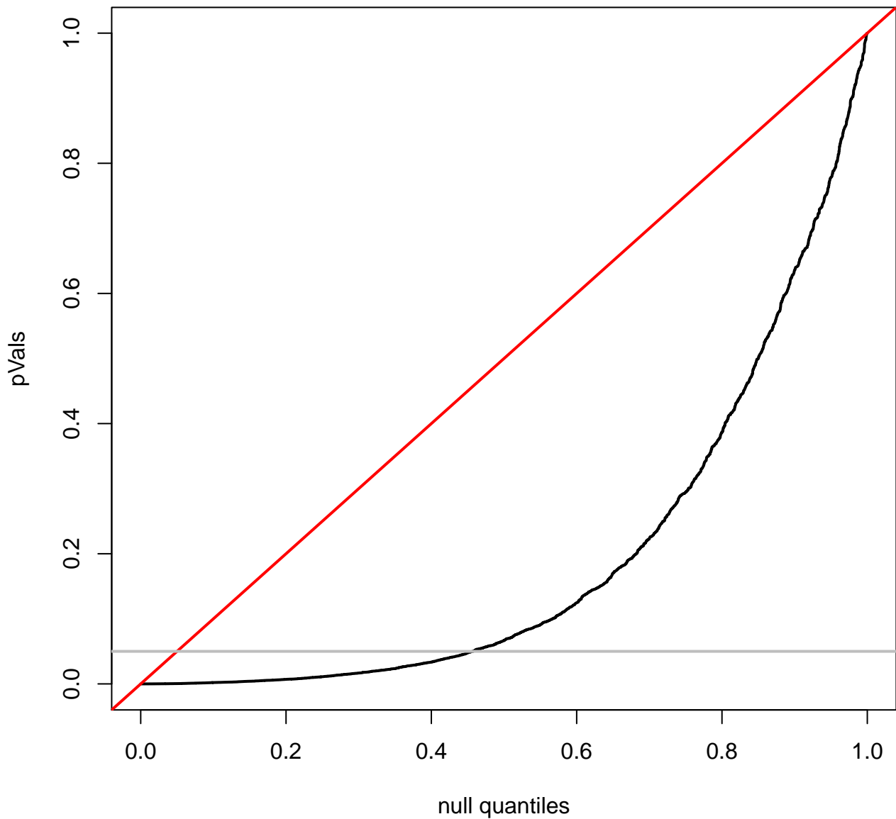
quantile plot for LUAD
