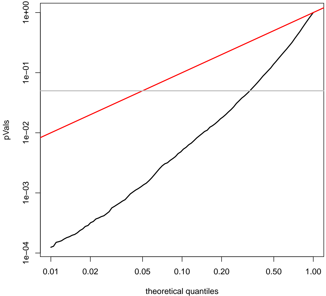
quantile plot for LHC (log-scale)
