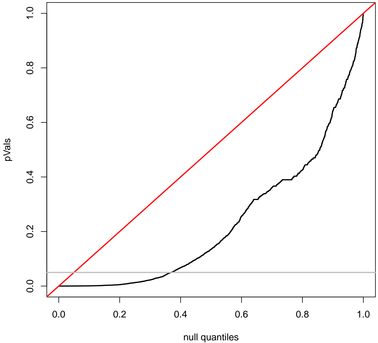
quantile plot for UVM
