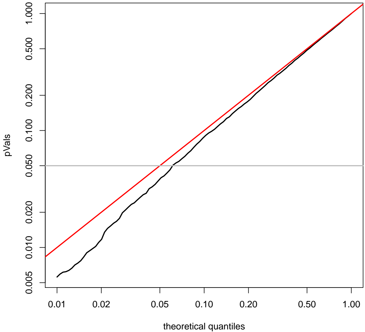
quantile plot for CESC (log-scale)
