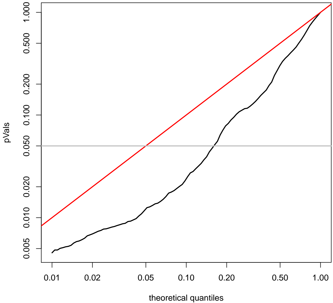
quantile plot for THYM (log-scale)
