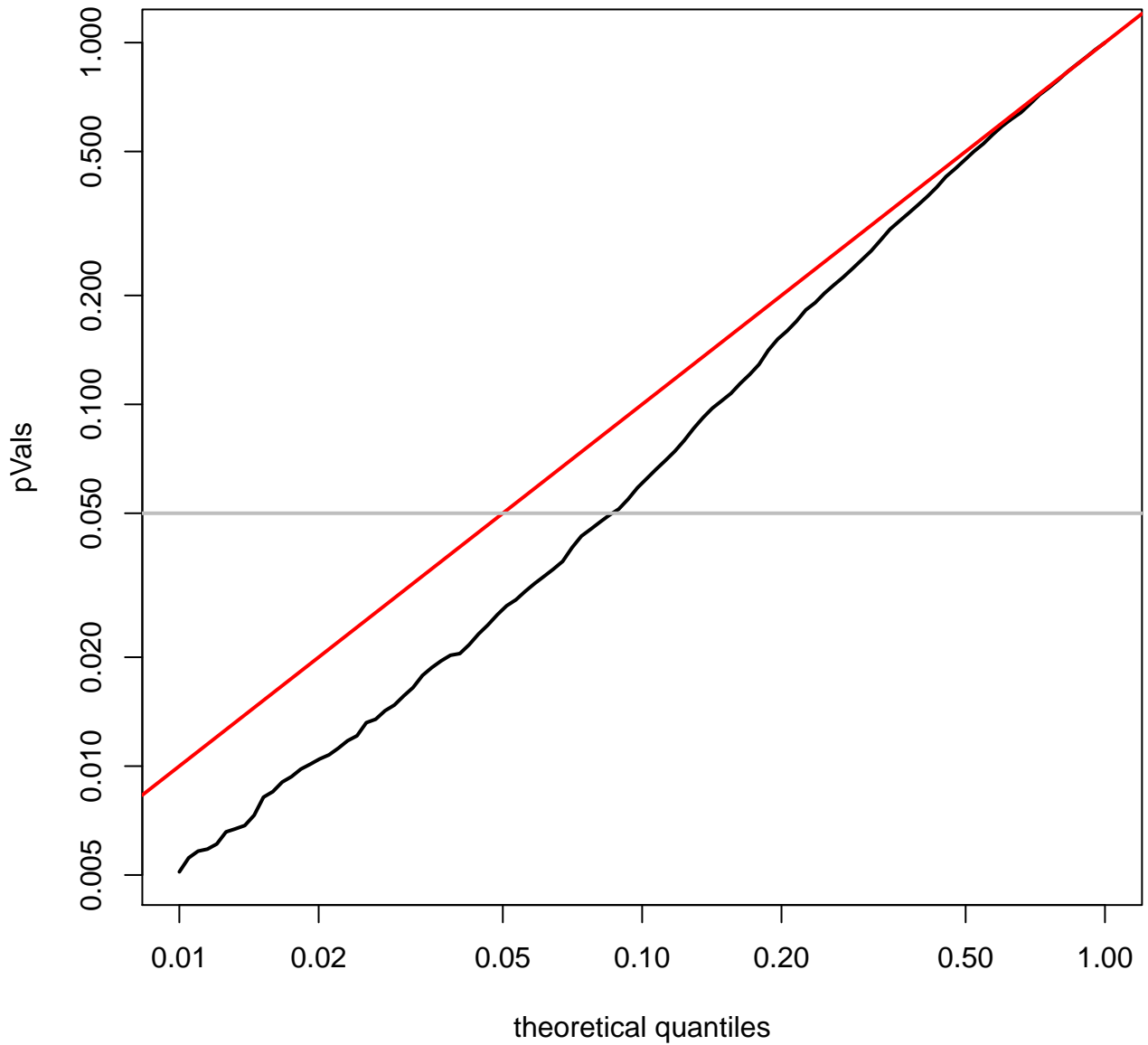
quantile plot for GBM (log-scale)
