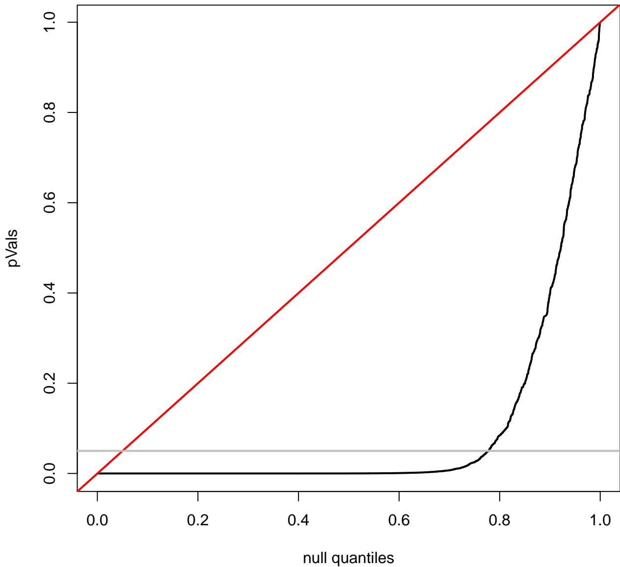
quantile plot for LGG
