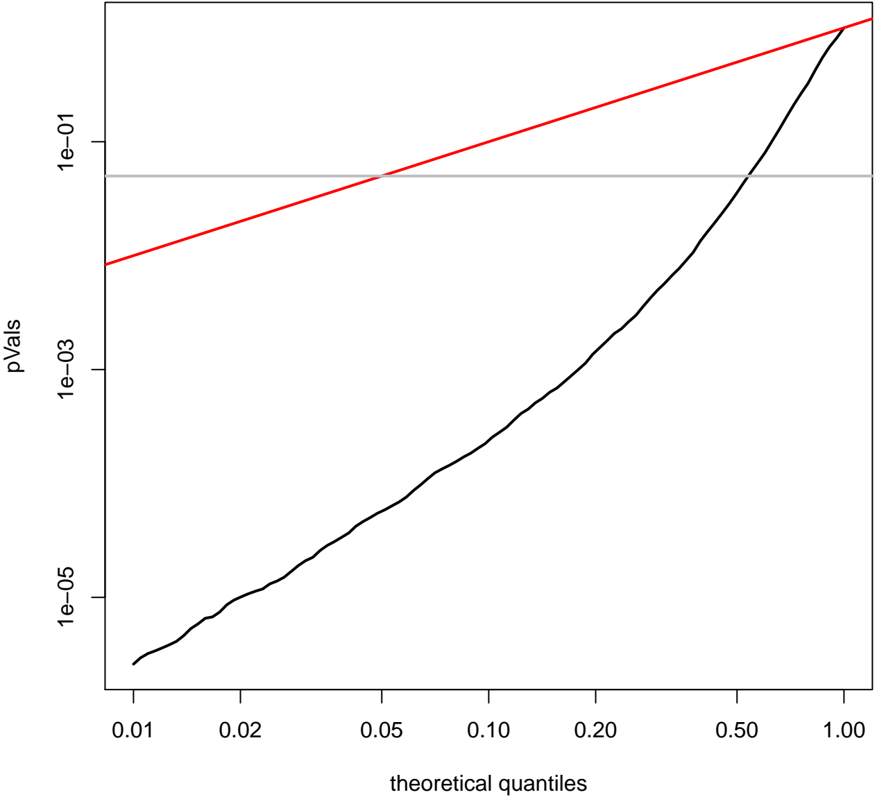
quantile plot for MESO (log-scale)
