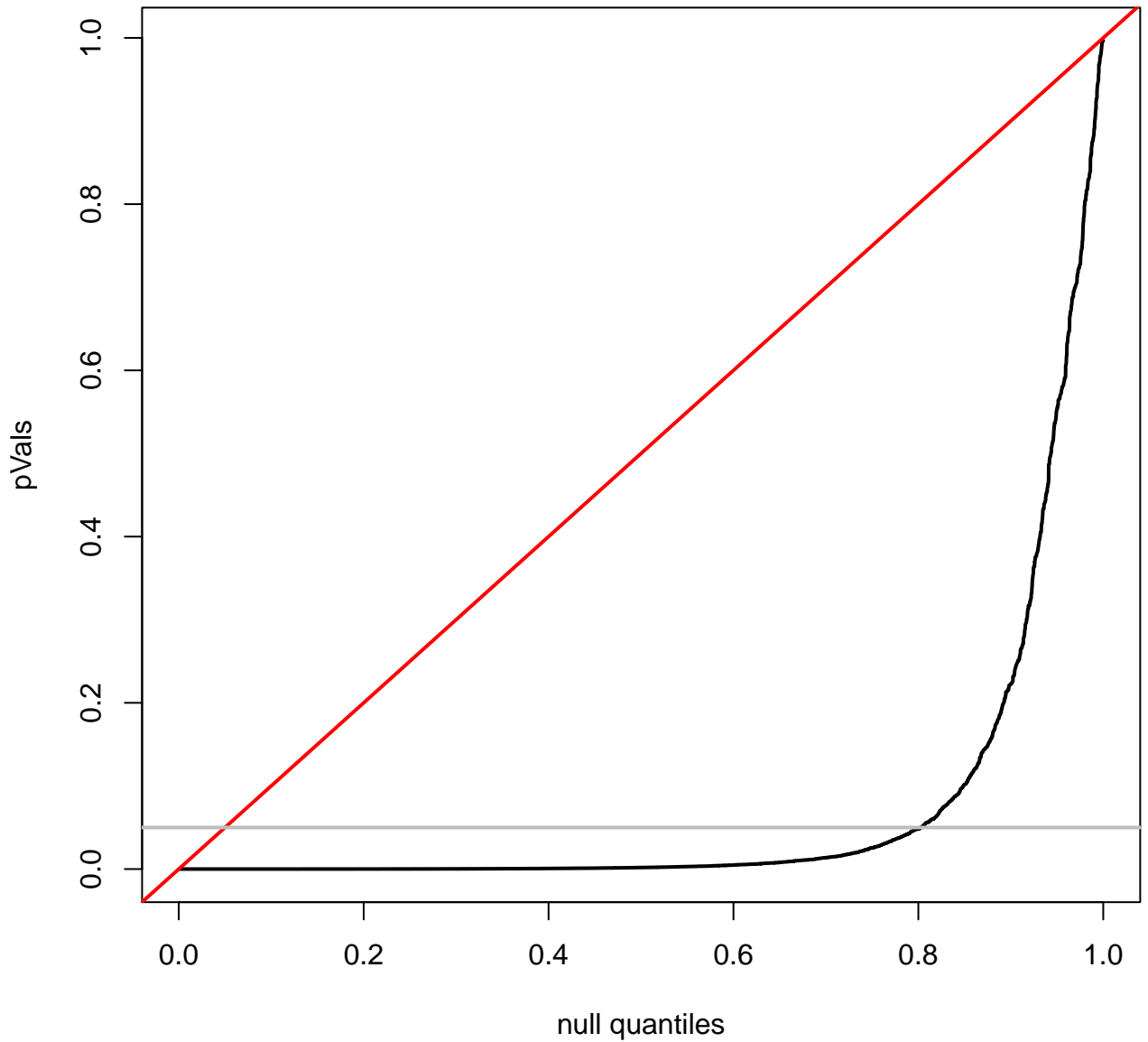
quantile plot for ACC
