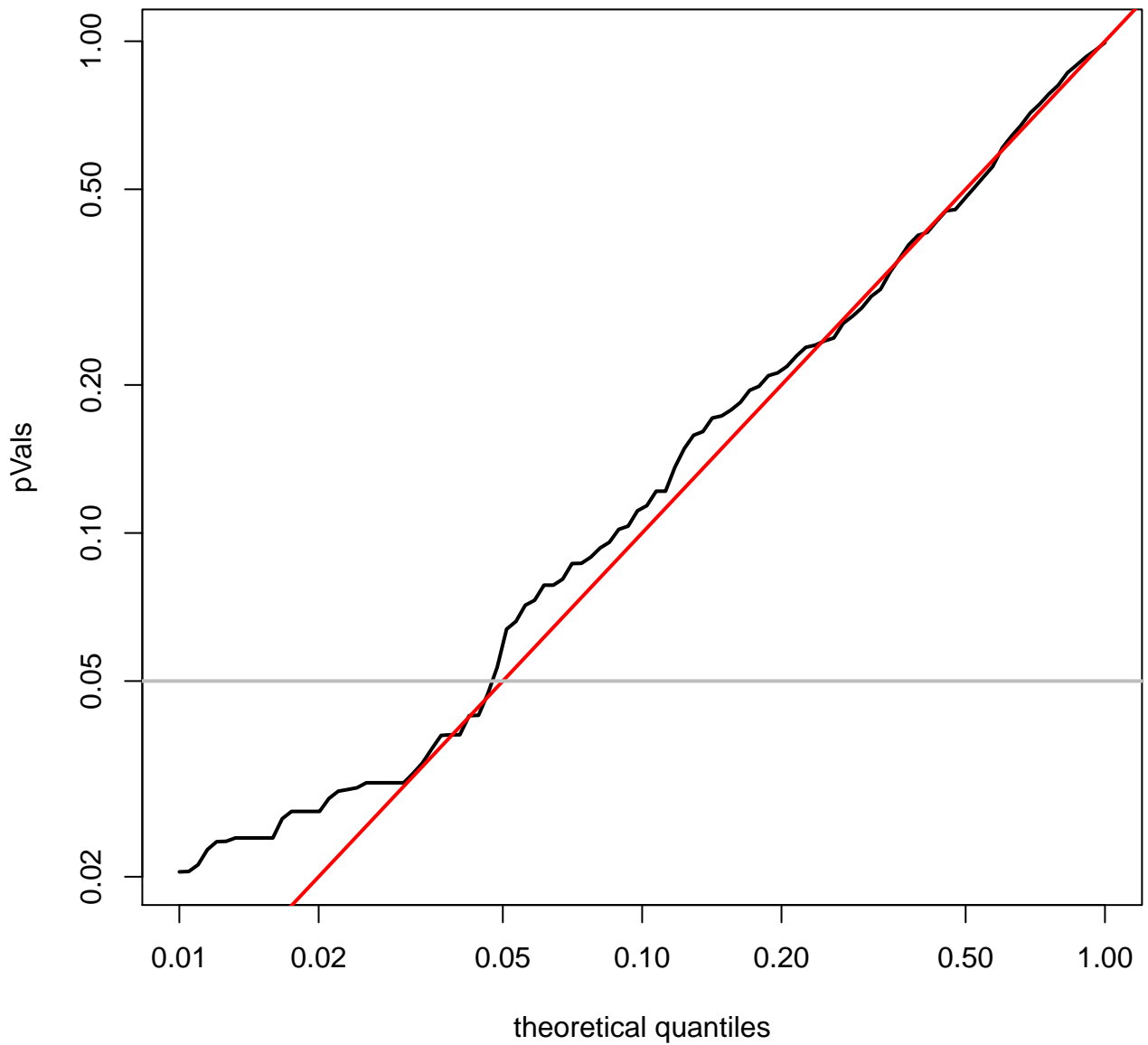
quantile plot for DLBC (log-scale)
