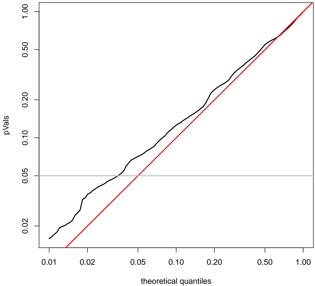
quantile plot for PCPG (log-scale)
