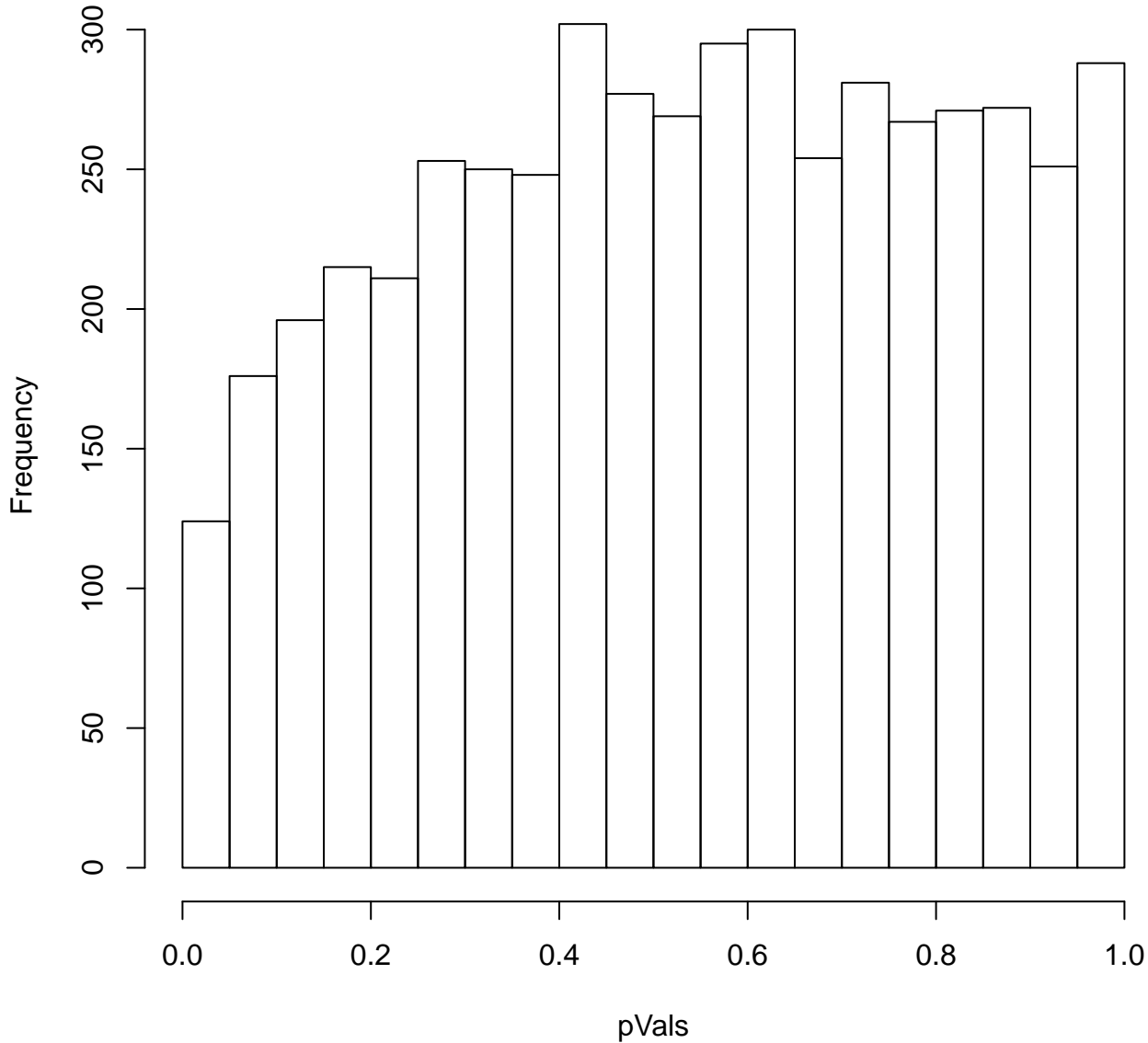
Histogram for pVals for COAD
