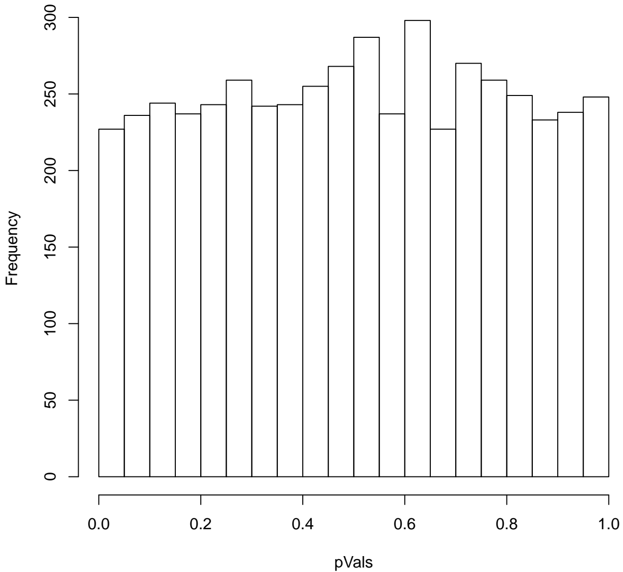
Histogram for pVals for OV
