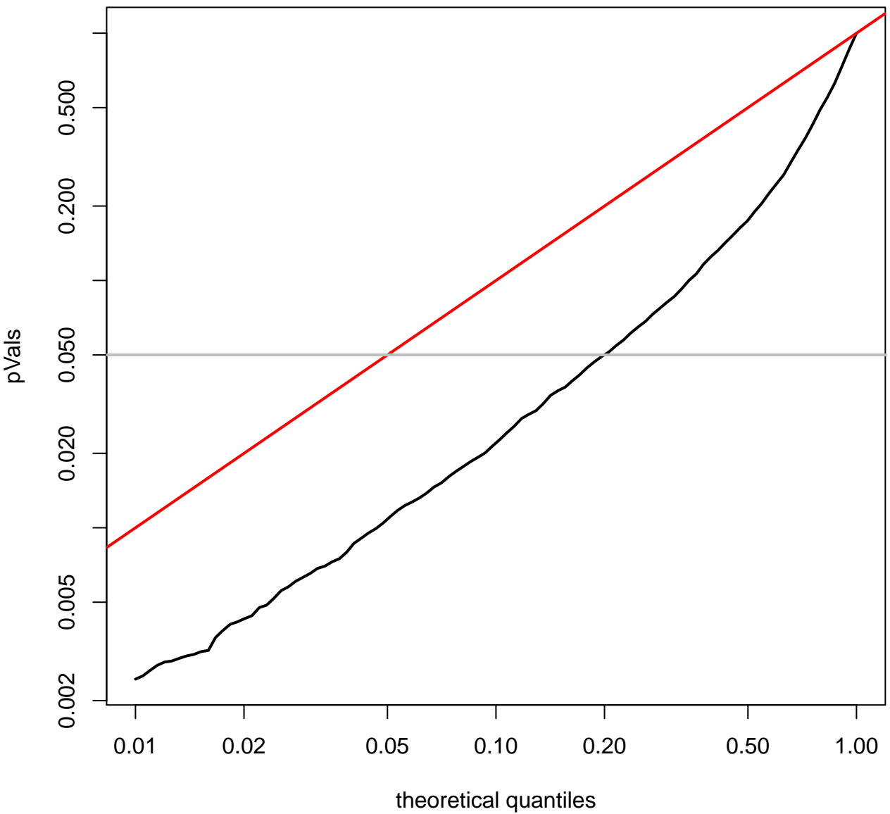
quantile plot for LUSC (log-scale)
