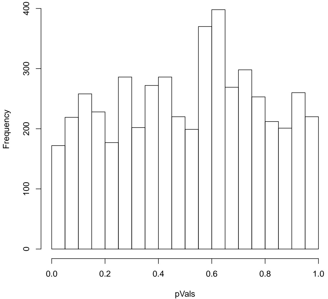
Histogram for pVals for PCPG
