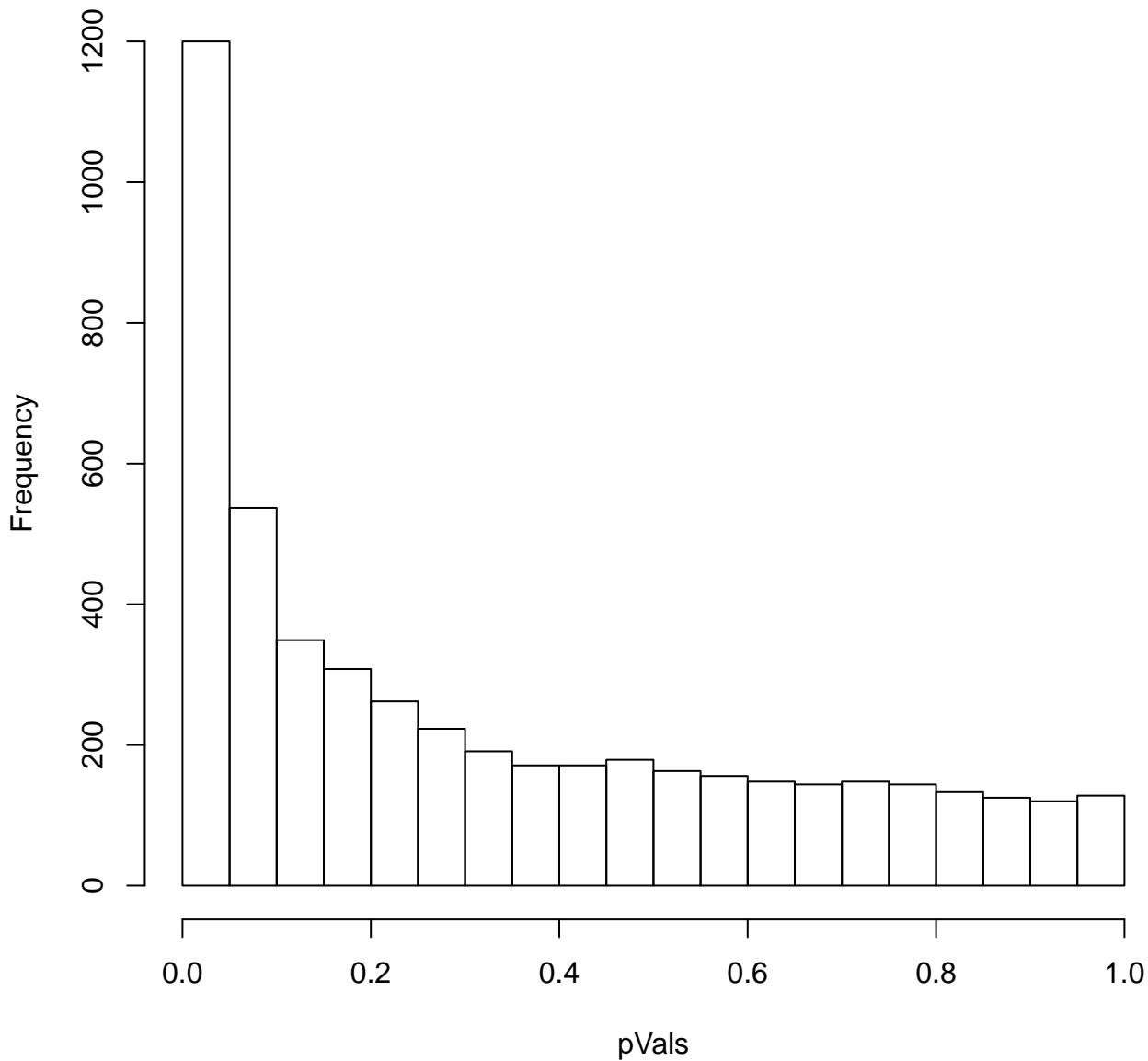
Histogram for pVals for HNSC
