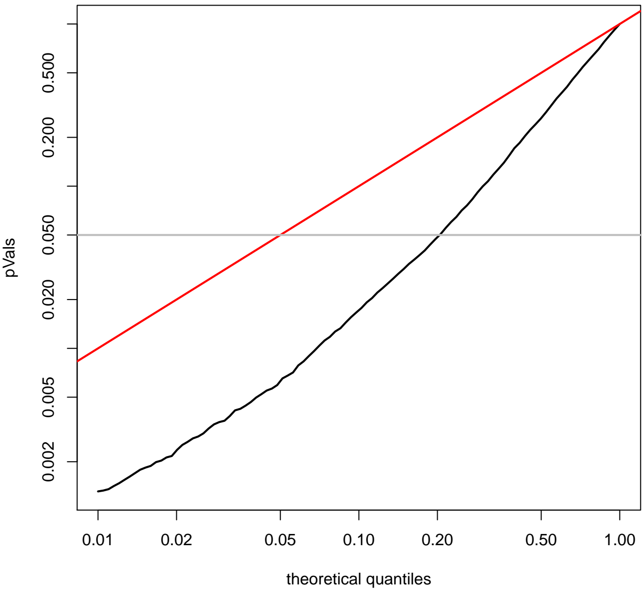
quantile plot for BRCA (log-scale)
