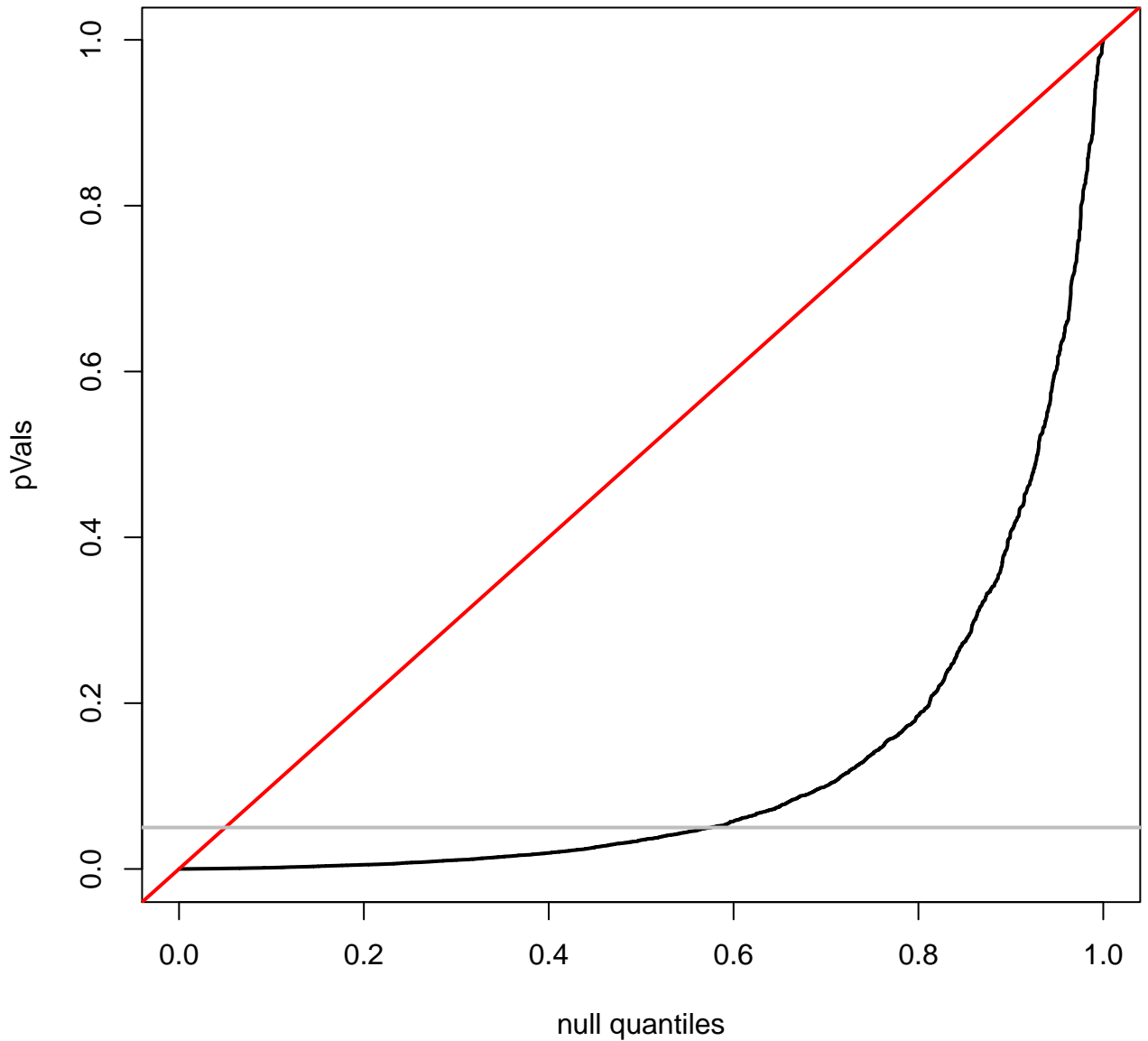
quantile plot for BLCA
