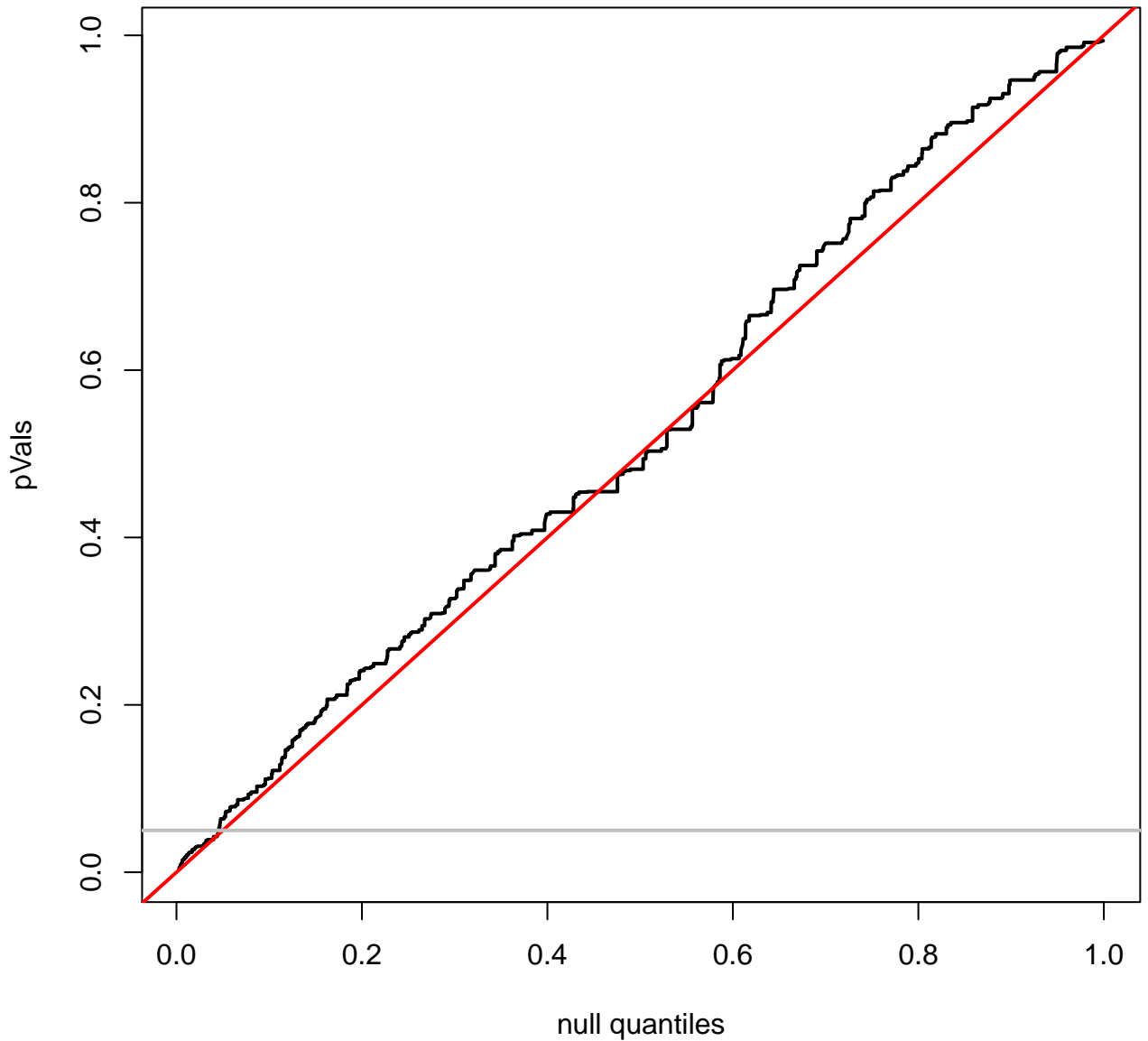
quantile plot for DLBC
