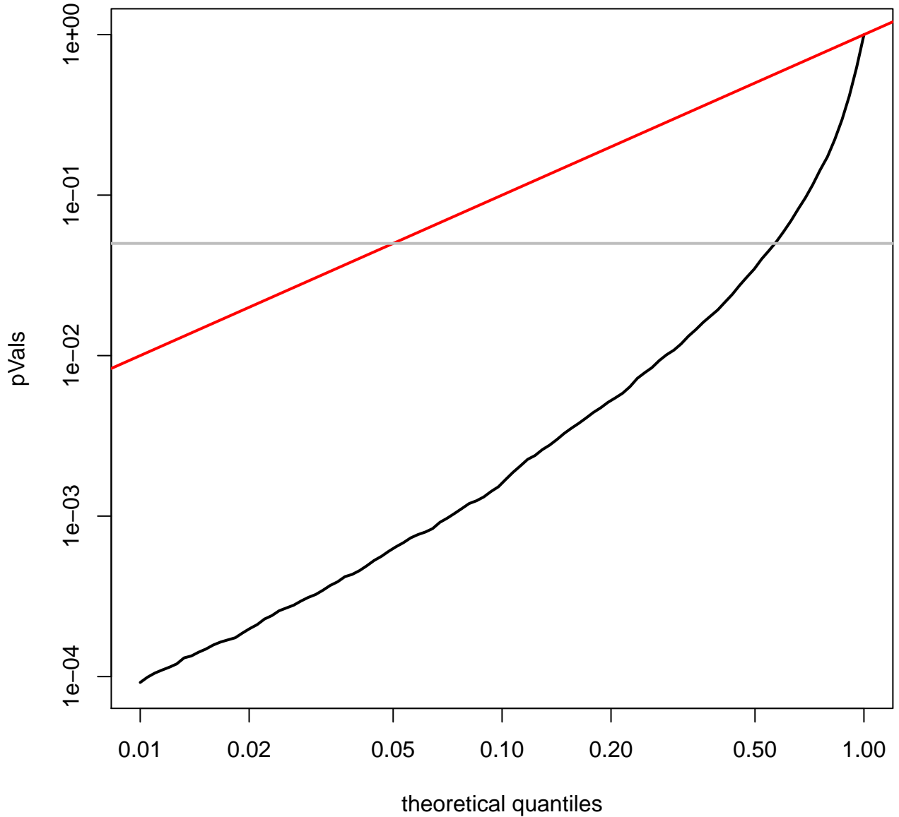
quantile plot for BLCA (log-scale)
