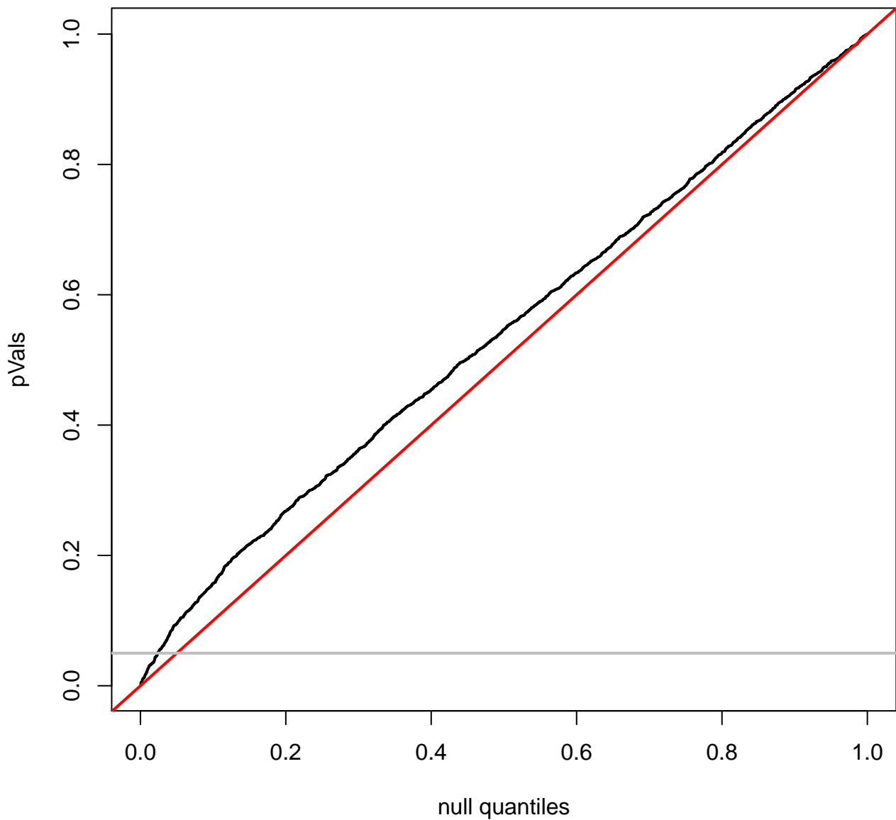
quantile plot for READ
