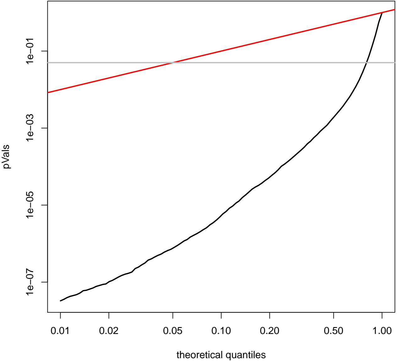
quantile plot for ACC (log-scale)
