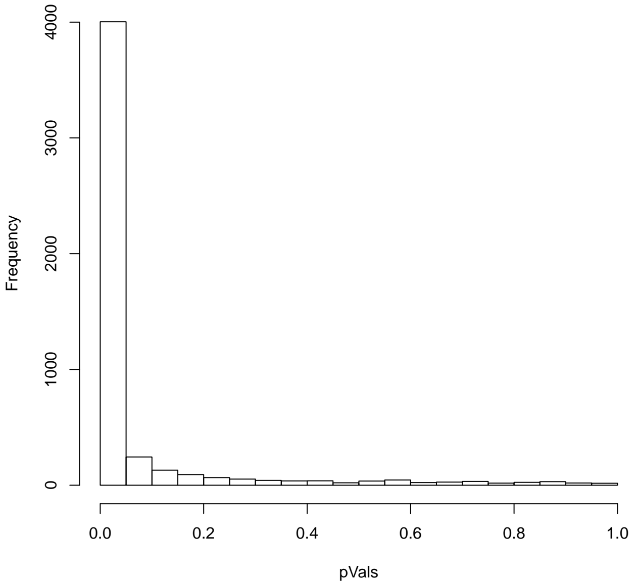
Histogram for pVals for ACC
