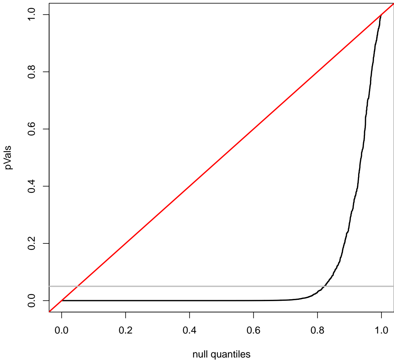
quantile plot for KIRC
