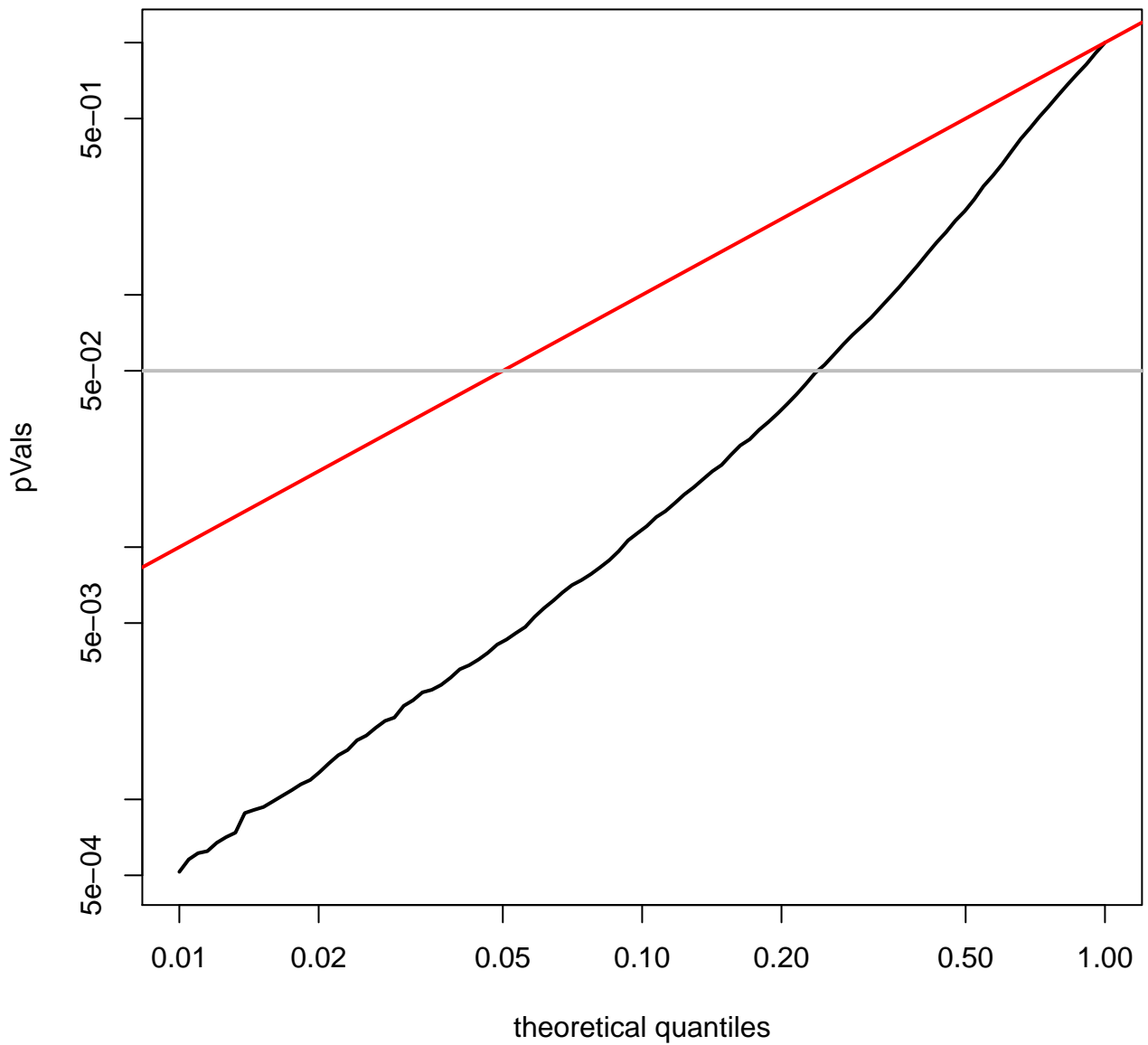
quantile plot for HNSC (log-scale)
