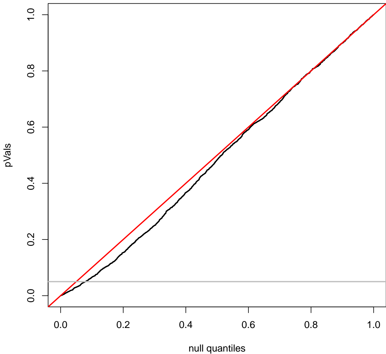
quantile plot for GBM
