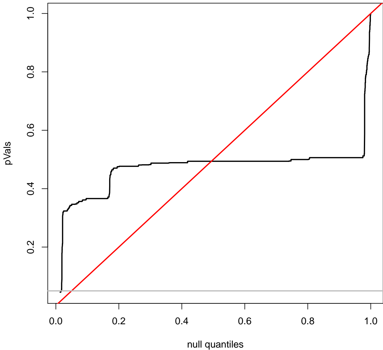
quantile plot for TGCT
