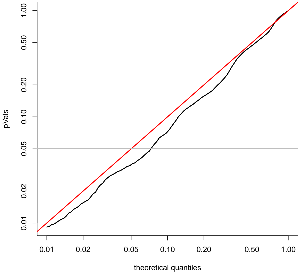
quantile plot for KICH (log-scale)
