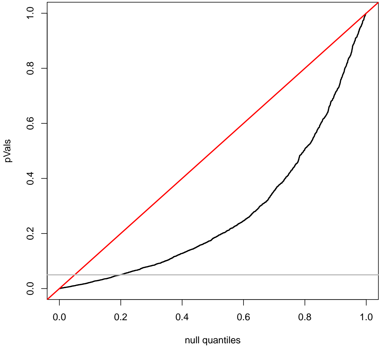
quantile plot for LUSC
