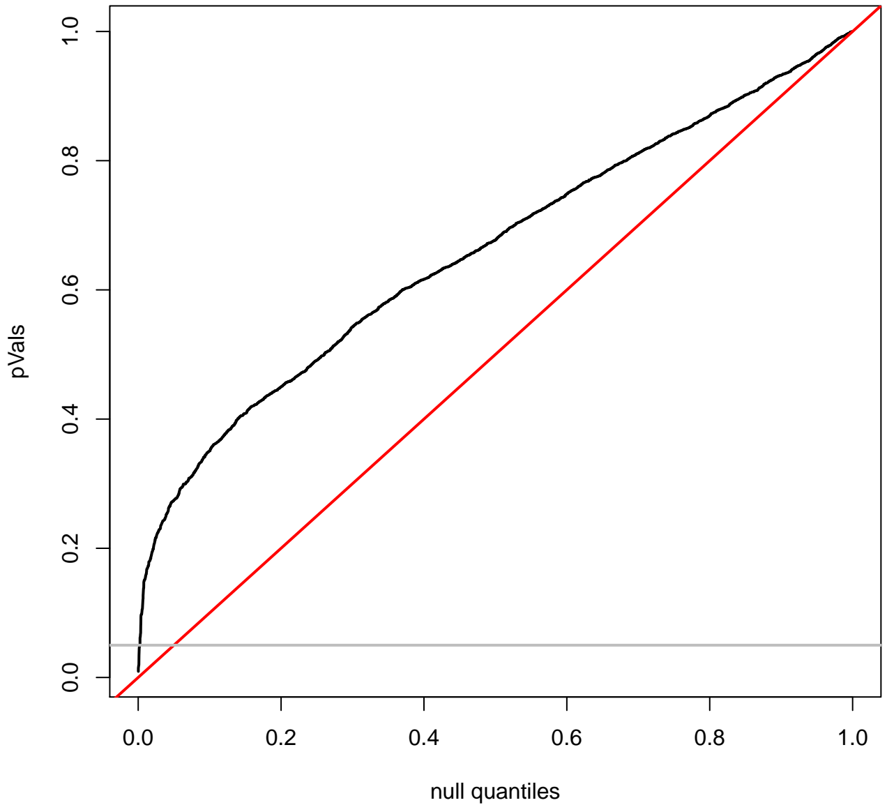
quantile plot for ESCA
