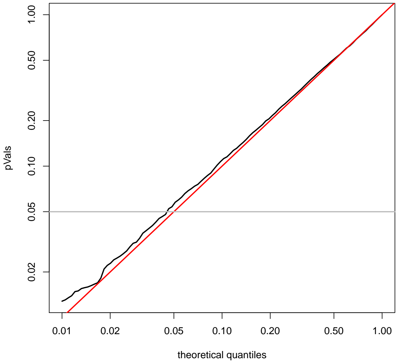
quantile plot for OV (log-scale)
