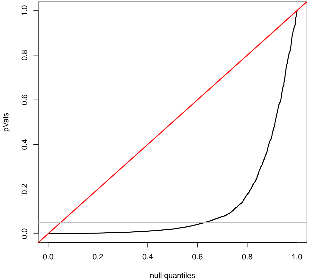
quantile plot for KIRP
