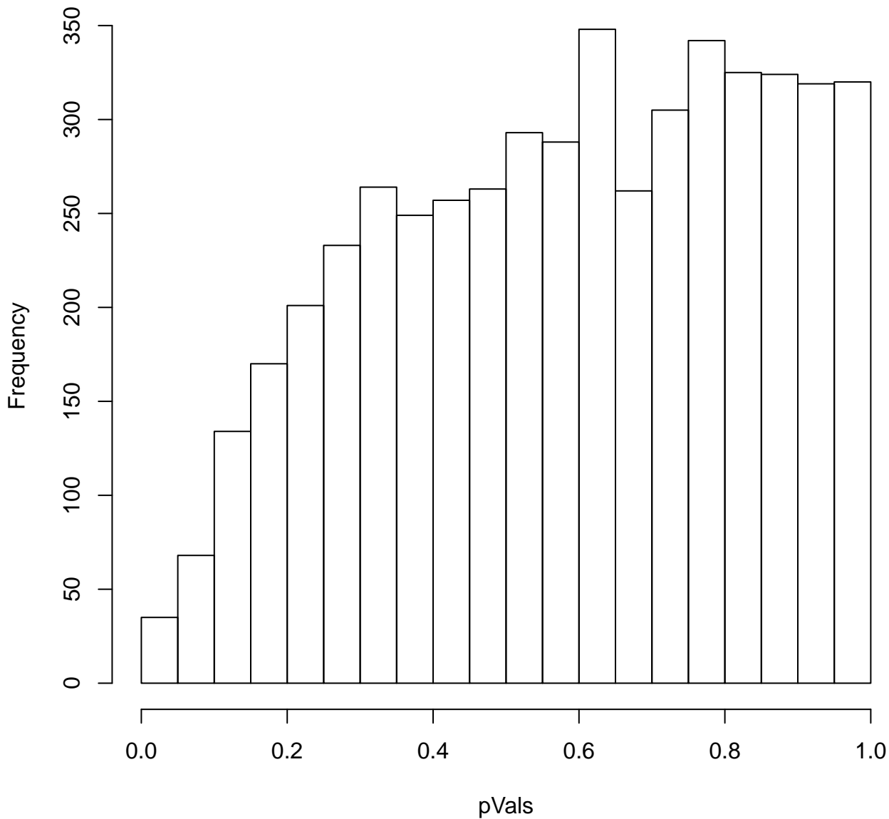
Histogram for pVals for CHOL
