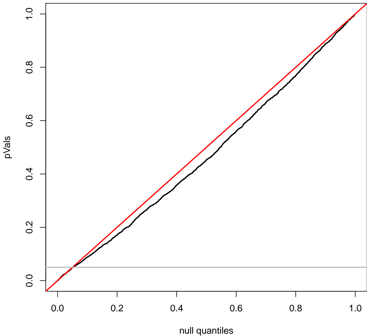
quantile plot for COADREAD
