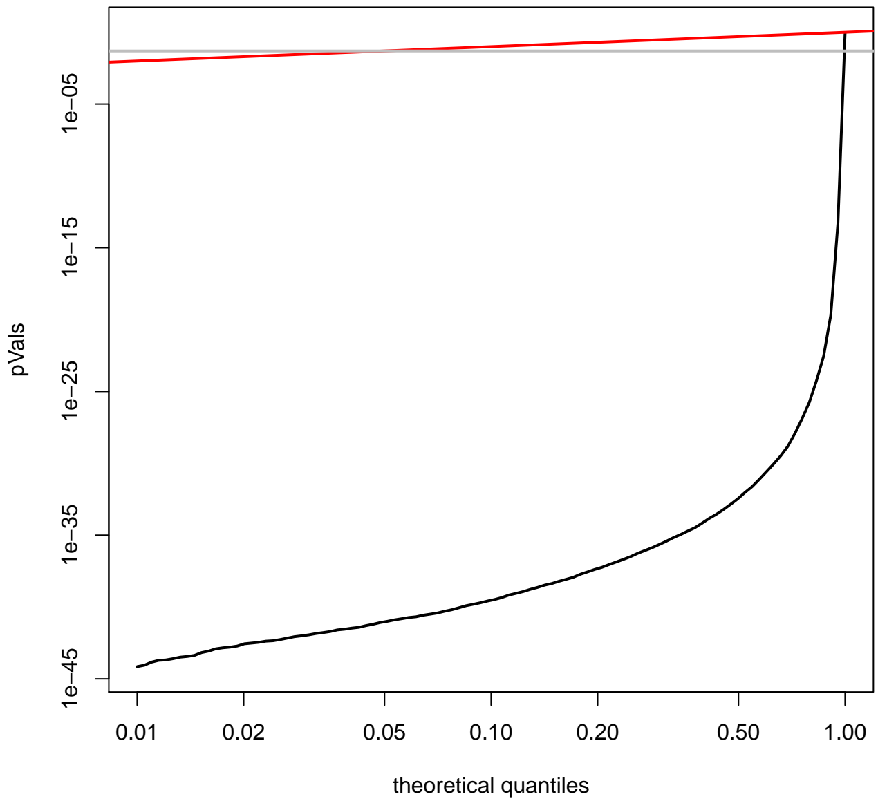
quantile plot for GBMLGG (log-scale)
