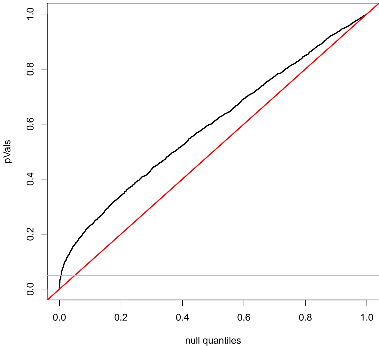
quantile plot for CHOL
