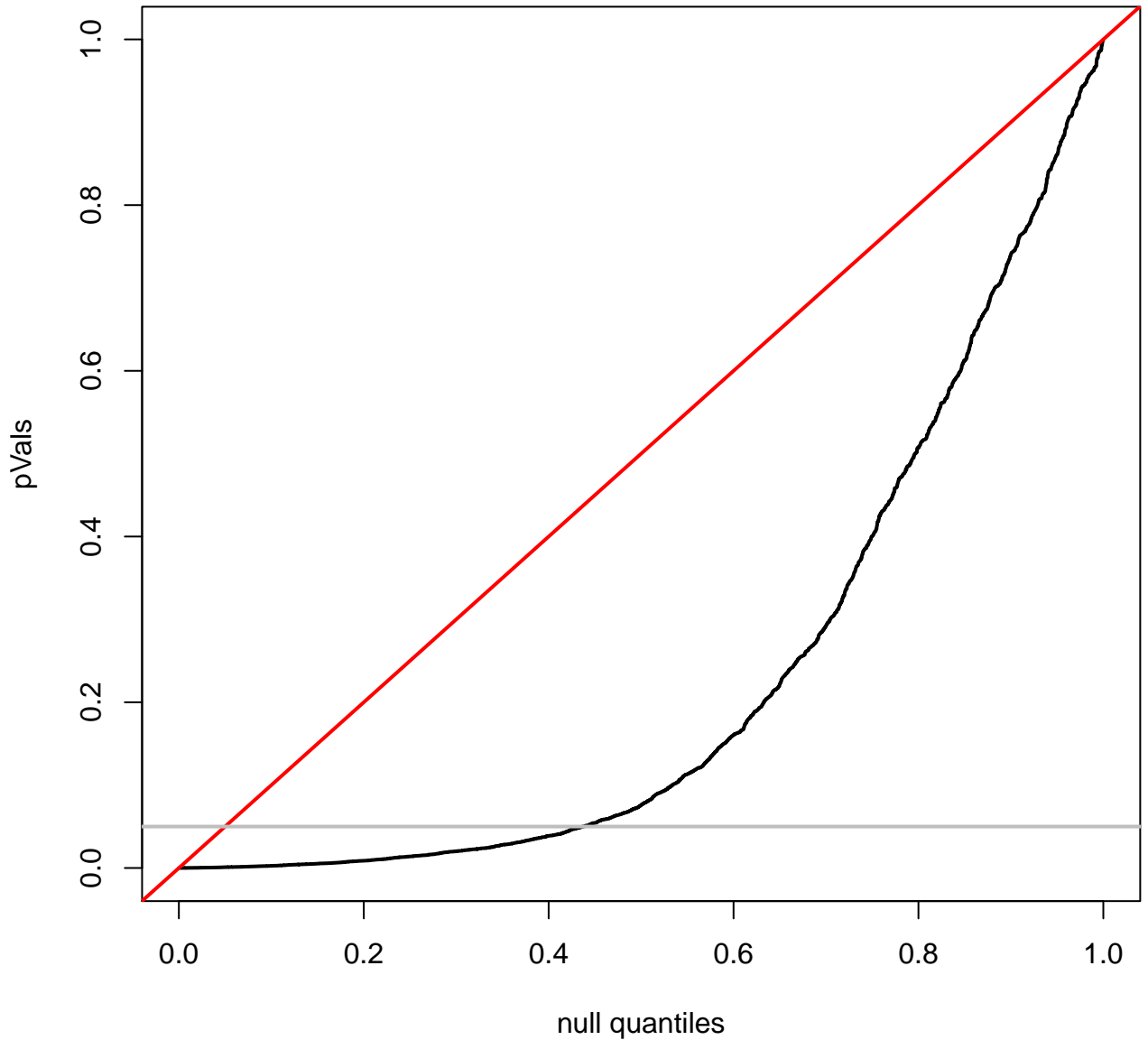
quantile plot for PAAD
