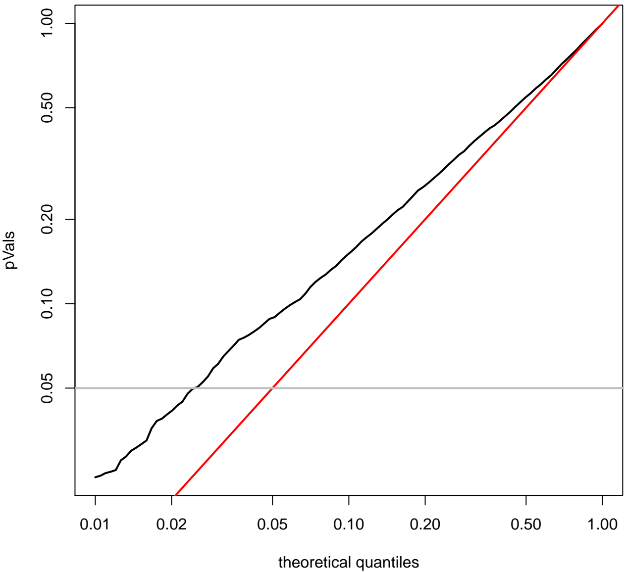
quantile plot for COAD (log-scale)
