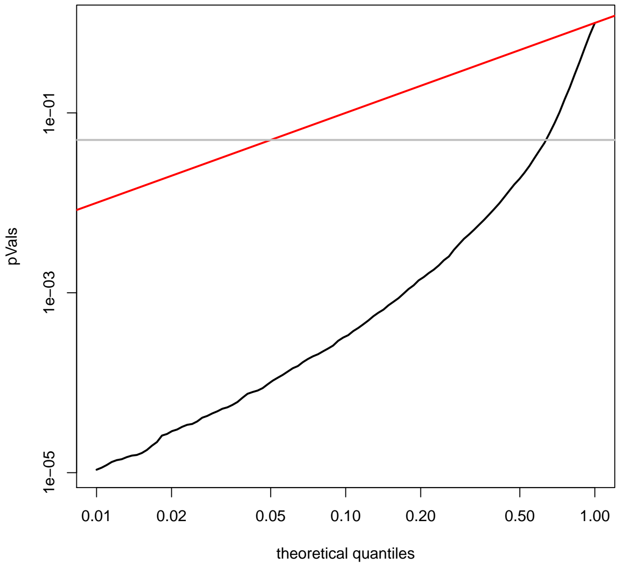
quantile plot for UCEC (log-scale)
