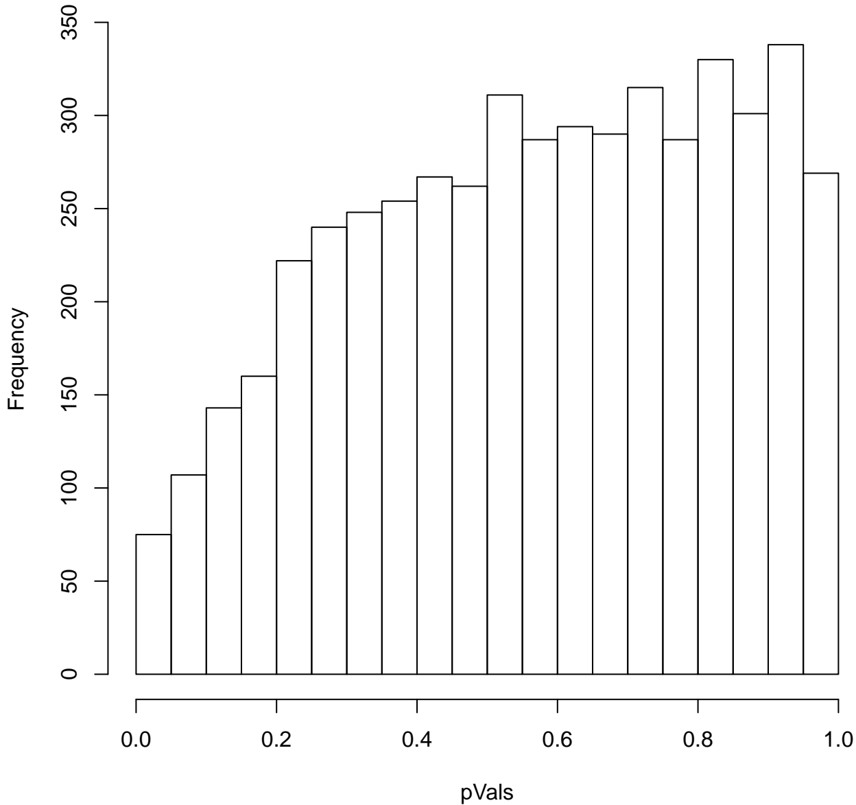
Histogram for pVals for UCS
