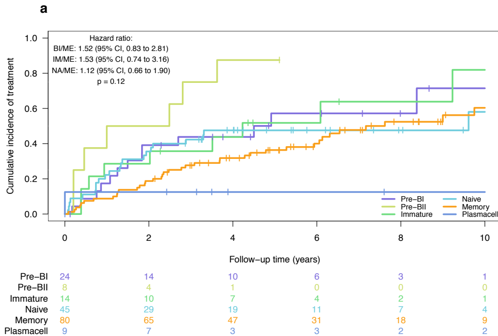
S5 Fig. Analyses of the prognostic impact of subtyping according to BAGS on TTT in watch-and-wait CLL. The cumulative incidence of treatment. (a) All subtypes. (b) All subtypes divided as early (pre-), naïve, and late (post-germinal). Only data from the IIDFCI, and UCSD cohort were used (n = 180), as the Munich cohort was excluded.
