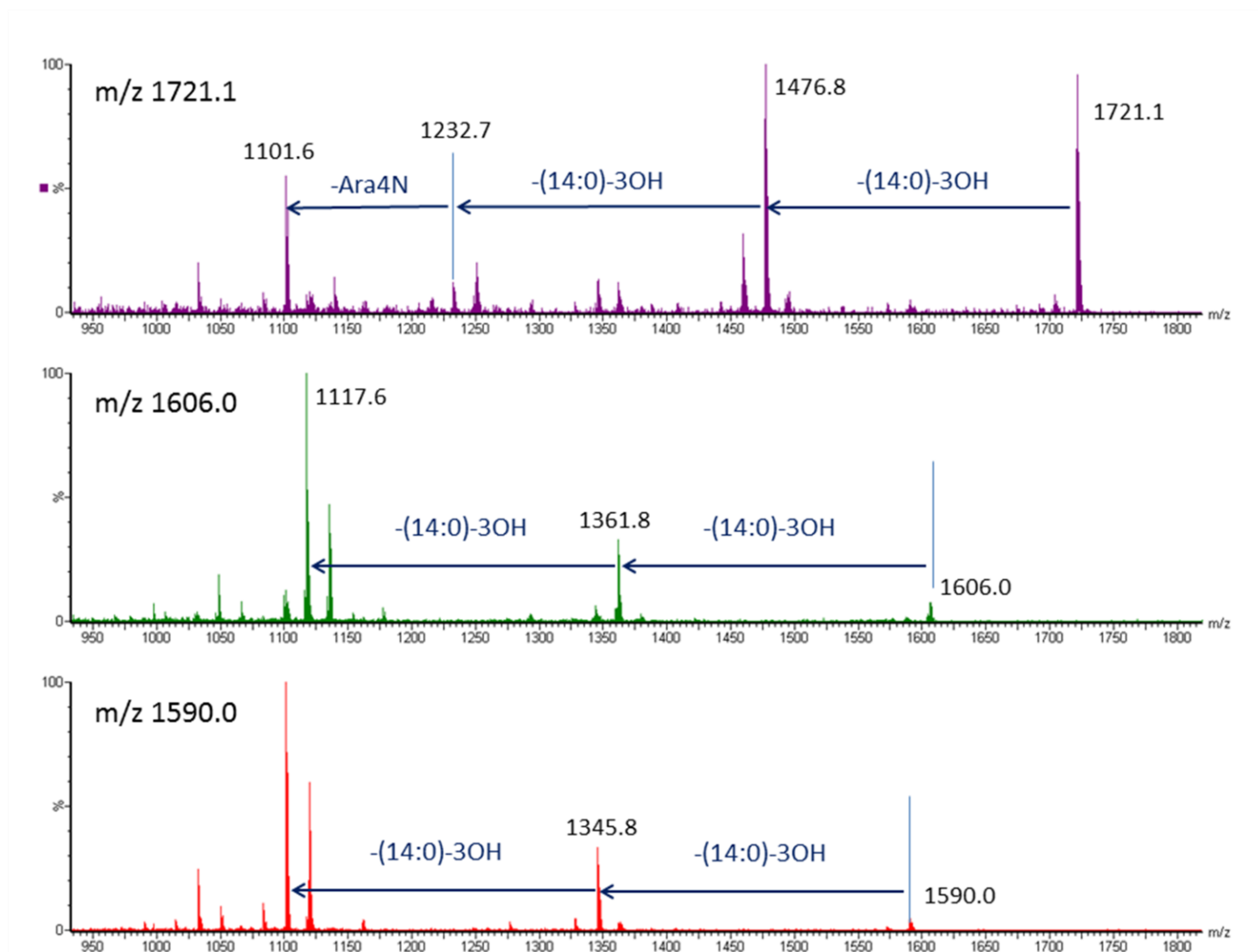
S1 Fig. Tandem MS spectra by ESI-QqTOF
