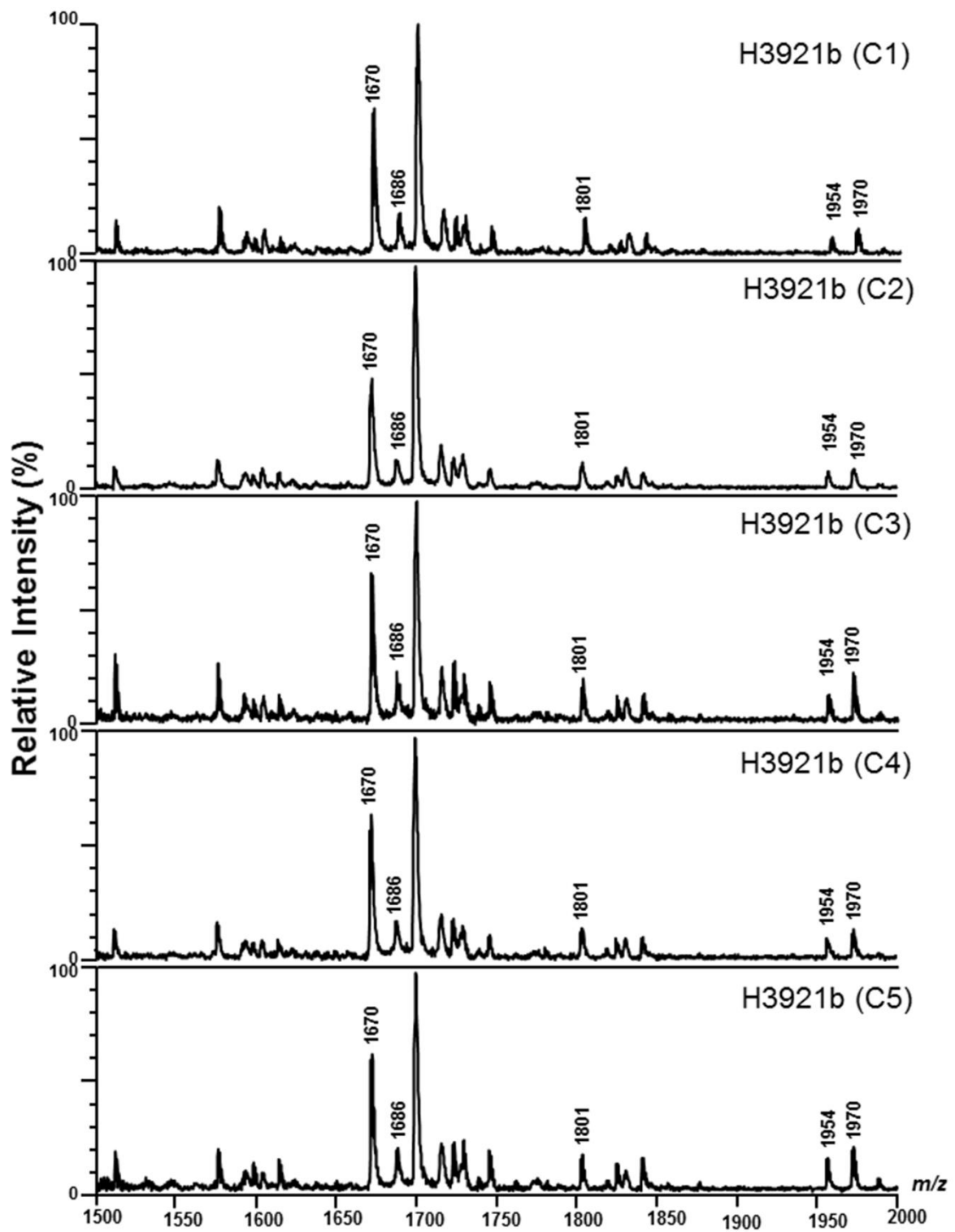
S4 Fig. MALDI-TOF lipid A spectra of 35 individual colonies of B. pseudomallei from 7 clinical specimens (5 colonies for each specimens) from a Thai patient with acute melioidosis
