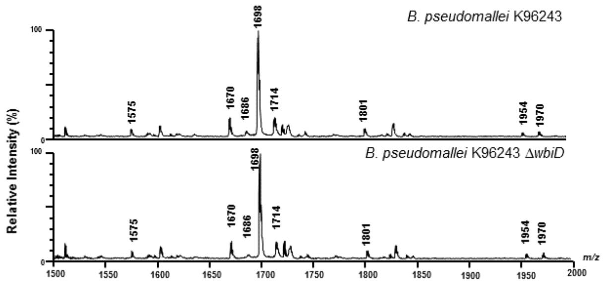
S6 Fig. MALDI-TOF lipid A spectra of B. pseudomallei K96243 and B. pseudomallei K96243 \Delta wbiD
