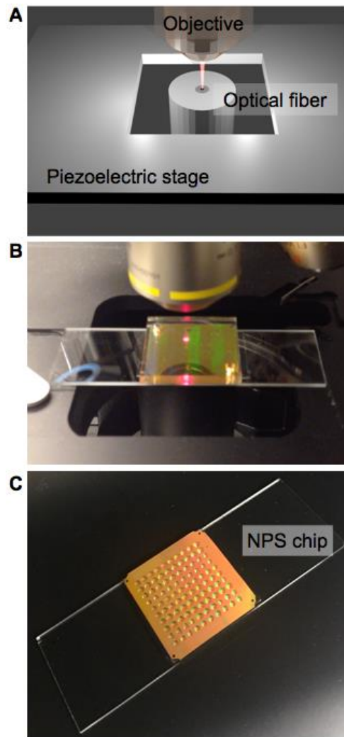
Fig. S1. NPS setup. (A) Schematics of NPS measurement setup on an upright microscope. (B) Photograph of NPS setup on a piezoelectric autostage. (C) Photograph of a NPS chip with 100 sensing arrays.
