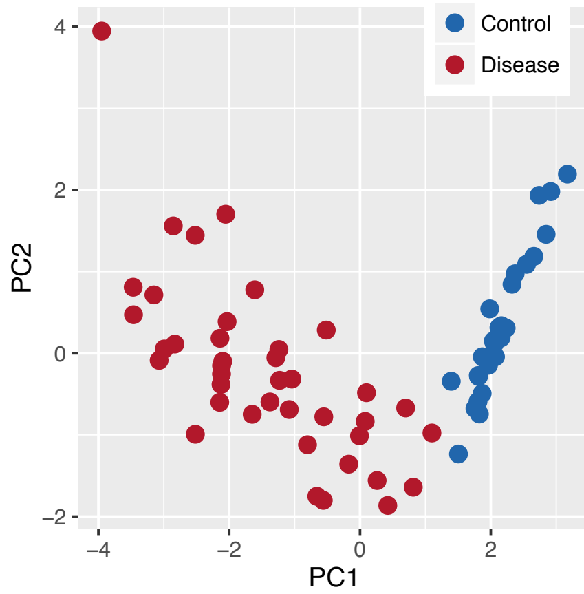
Figure S1. Principal Component Analysis of a subset of the DMD dataset that includes only the 6 proteins in the short biomarker panel.
