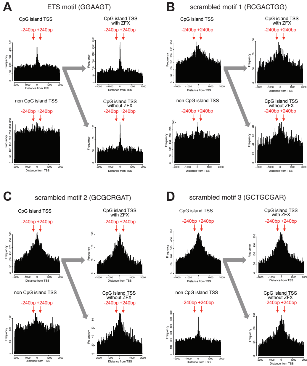
Supplemental Figure S2. Scrambled ZFX motifs are not enriched at \pm 240 bp of the TSS. Shown is the frequency at which the ETS motif GGAAGT, as an example of a known motif for a TF other than ZFX that binds to promoter regions (A), scrambled ZFX motif 1 (B), scrambled ZFX motif 2 (C), or scrambled ZFX motif 3 (D) are located \pm 2 kb from the TSS of CpG island promoters, of non-CpG island promoters, of CpG island promoters bound by ZFX, and of CpG island promoters not bound by ZFX.
