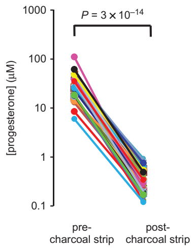
Supplementary Figure S1 Concentrations of P4 in 31 hFF samples assessed before (left) and after (right) stripping of lipid-derived molecules with dextran-coated charcoal. hFF, human follicular fluid.
