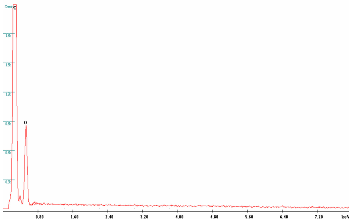
Figure S1. EDX spectrum of chitin isolated from M. euplectellioides demosponge. Spectrum was registered with use of a XL 30 ESEM Philips-Scanning Electron Microscope (Netherlands). The uncoated samples were investigated at an accelerating voltage of 20 kV.
