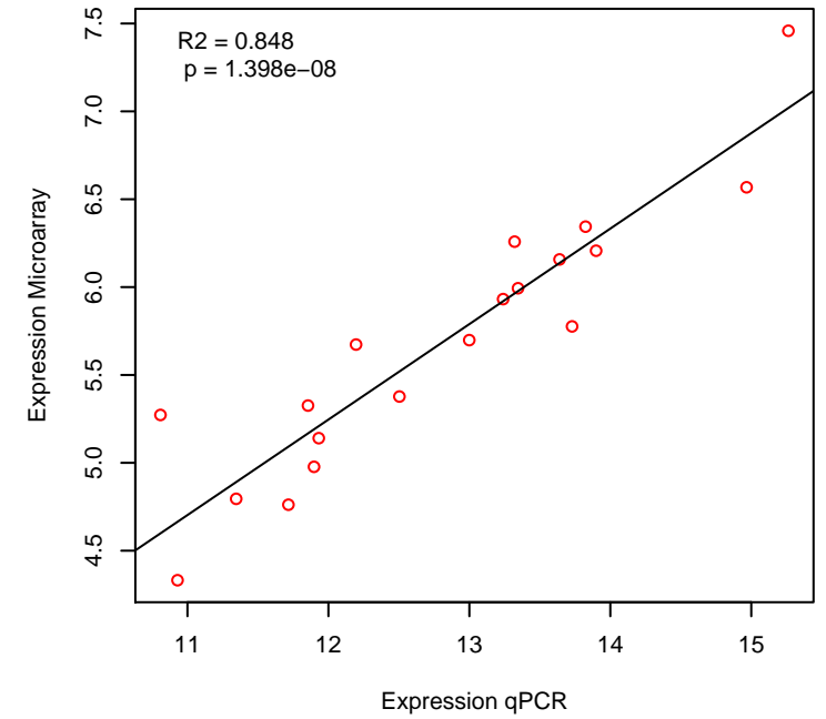
MMP2
