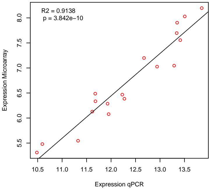
c1s
