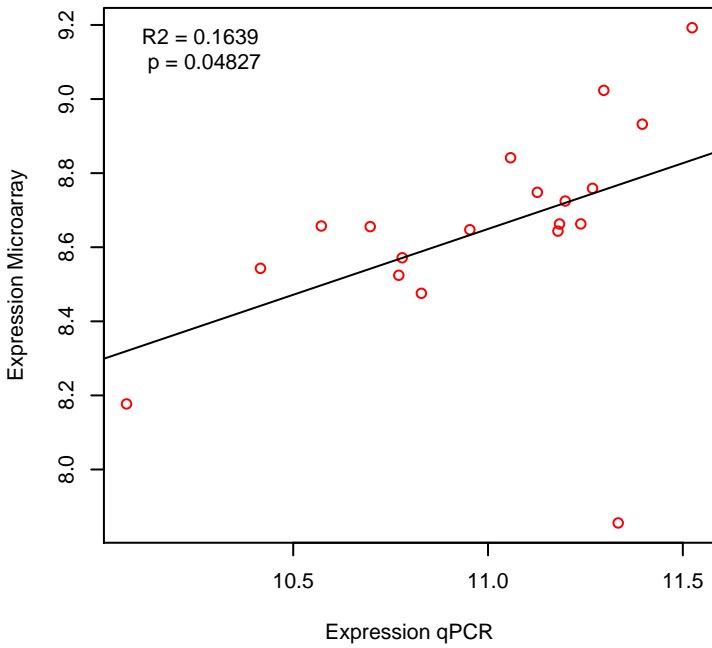
SLC34A3
