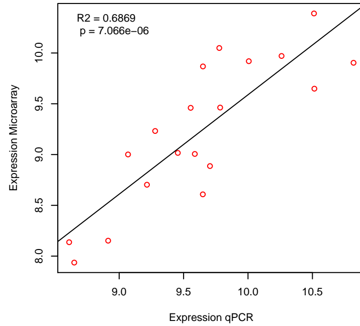
C1QC
