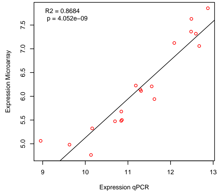
c7
