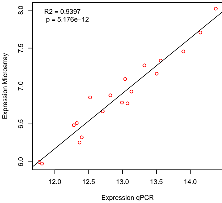
CYP27A1
