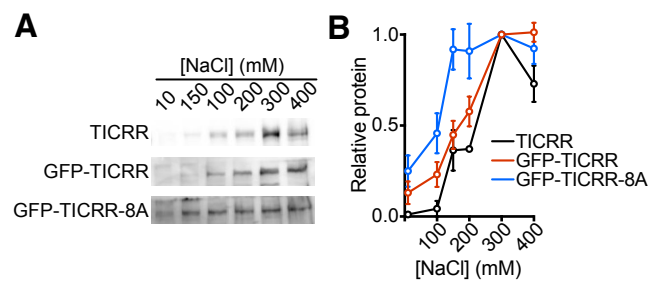
Fig. S4. The TICRR-8A mutant is extracted from nuclei at lower salt concentrations than wild-type TICRR. (A) Immunoblots showing the amounts of endogenous TICRR, EGFP-TICRR, or EGFP-TICRR-8A that was extracted from U2OS nuclei using the indicated NaCl concentrations. (B) Quantification of (A) with triplicate experiments. Mean \pm SD is shown.
