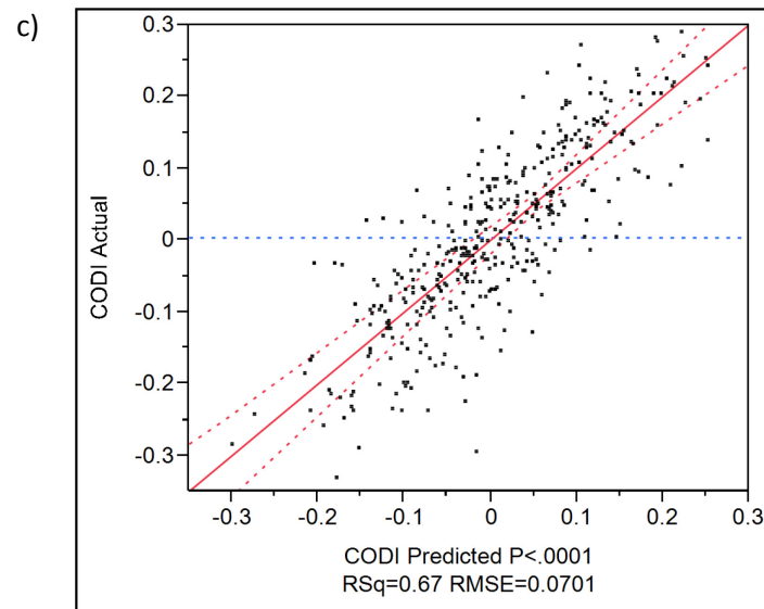
Supplementary Figure 2. Modelling cookie diameter using only QTLs (a), phenotype data (b) and QTL + phenotype data (c) in panel of soft winter wheat. The quality traits and their respective QTLs used include: single kernel hardness, cookie diameter, break flour yield, total flour yield, flour ash content, lactic acid SRC, water absorption SRC and carbonate SRC.
