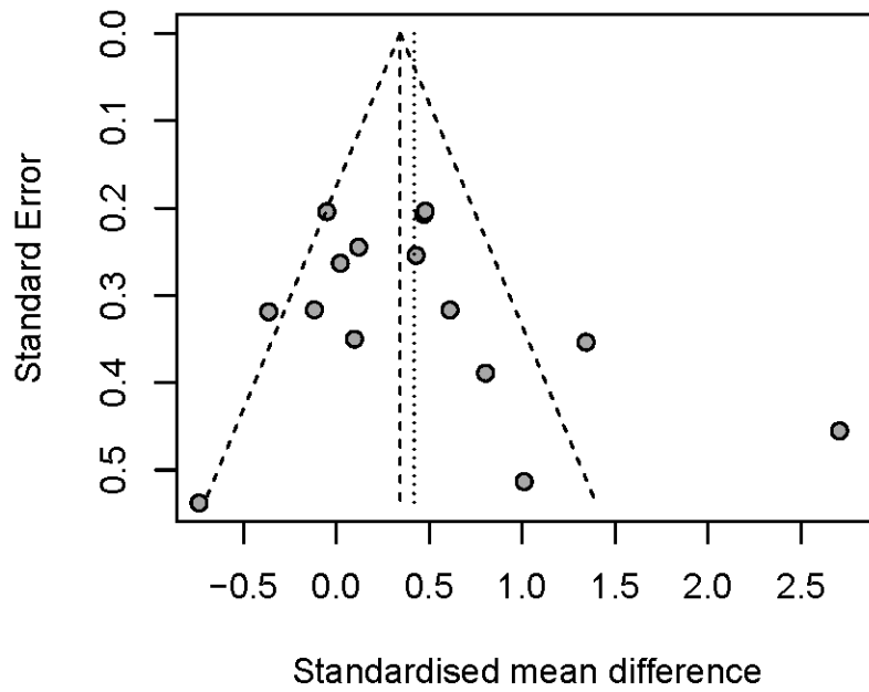
Figure S1. Bias assessment plot for ALB level at week 4
