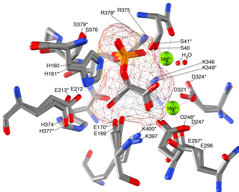
Figure S12. Structural comparison of catalytic sites of CaEno1 and ScEno1 polypeptides bound to phosphoenolpyruvate/2-phosphoglycerate. Surface of substrate/product is represented by a mesh. Asterisks, residues corresponding to C. albicans enolase 1.
