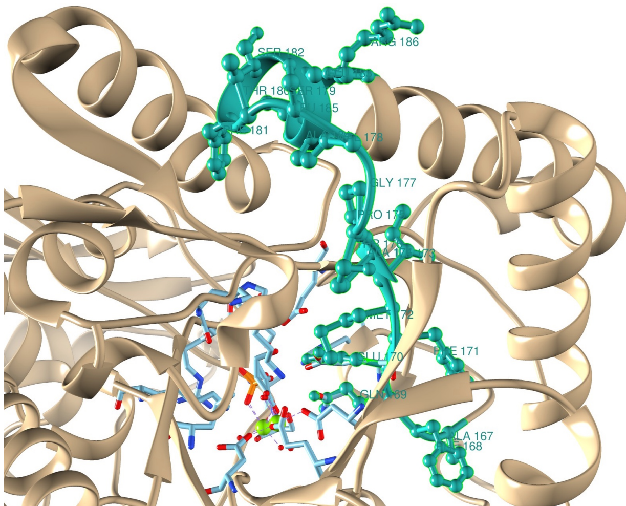
Figure S14. Identification of a putative TGase active site in the CaEno1 structure (green), showing the peptide AFQEFMIAPTGVSTFSEALR (residues 167-186) that corresponds to the PROSITE PS00547 TGase active ([GT]-Q-[CA]-W-V-x-[SA]-[GAS]-[IVT]-x(2)-T-x-[LMSC]-R-[CSAG]-[LV]-G) ( http://prosite.expasy.org/PS0054 ).
