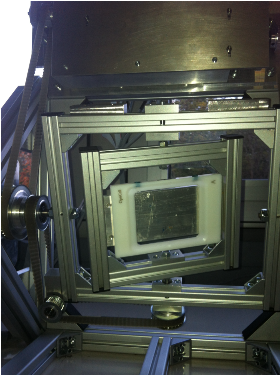
Figure S1. Image of the custom Random Positioning Machine. The dimensions of the 3D-clinostat are 50x50x70 cm with an inner and outer frame, which are independently controlled by the motors. The vials containing the samples were immobilized on the center of the platform located on the inner frame.
