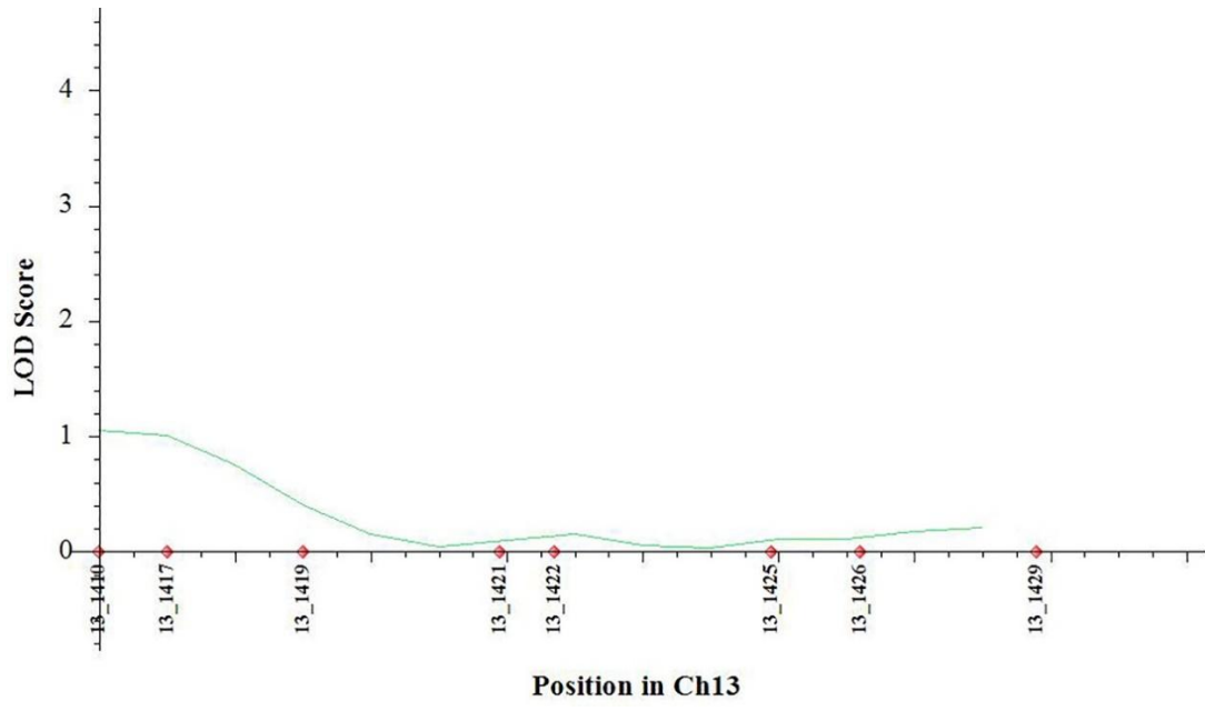
Fig. S1 Distribution of the LOD scores for days to flowering in the target region detected by QTL-seq.
