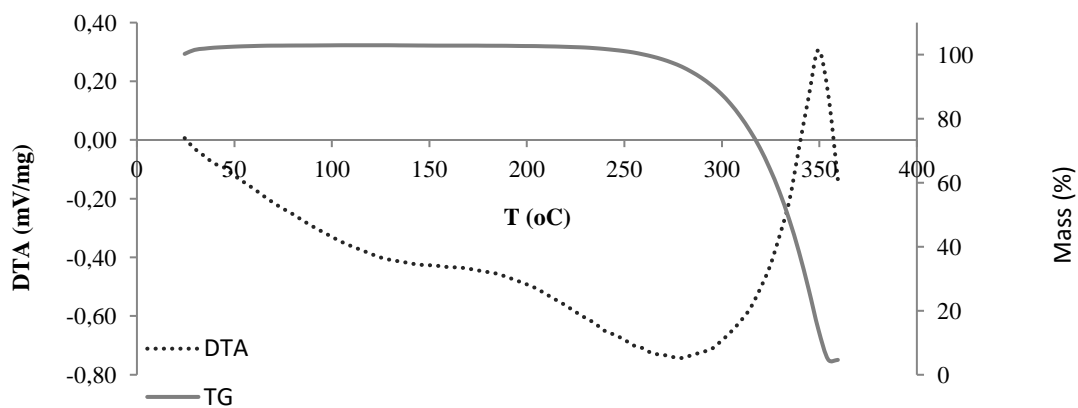
Figure S2. MEM thermogravimetric and differential thermal analysis.
