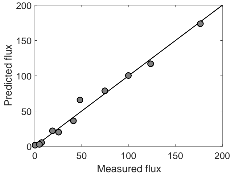
Figure S10: Comparison of predicted and measured intracellular fluxes for eleven reactions in carbon central metabolism ( \text{EX}_{glc} , PGI, G6PDH2r, PGMT, GAPD, PYK, PDH, PPC, MDH, TKT1, and TKT2) of E. coli . Fluxes are given relative to the specific glucose consumption rate.
