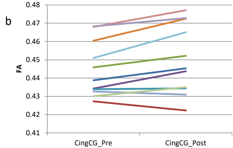
Figure S 2: Within subject changes in FA at the a) body of corpus callosum b) cingulate gyrus and c) forceps minor. Each line represents the FA of each of the 11 patients. The increase in FA was observed across majority of patients . FA, fractional anisotropy; BodyCC_Pre, FA at the body of corpus callosum pre-transplant; BodyCC_Post, FA at the body of corpus callosum post-transplant; CingCG_Pre, FA at the cingulate gyrus pre-transplant; CingCG_Post, FA at the cingulate gyrus post-transplant; Fmi_Pre, FA at the forceps minor pre-transplant; Fmi_Post, FA at the forceps minor post-transplant.
