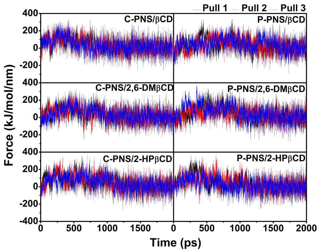
Fig. S1 The force-time profile of the ligand being pulled out from the wider rim along the host cavity axis for each inclusion complex
