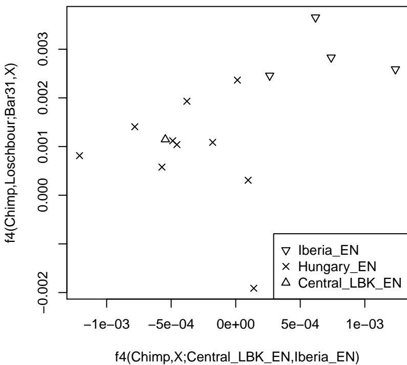
Early Neolithic, rho=0.52143; p=0.04883
