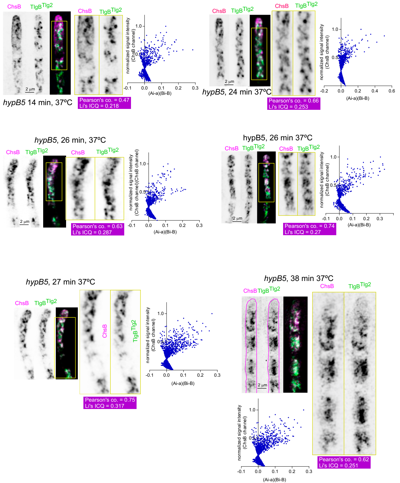
S2 Figure. Colocalization analyses of mCh-ChsB and GFP-TlgB Tlg2 in a hypB5 (sec7 ts ) strain Pictures taken at different times after shifting cells at 37°C, with indication of Pearson's and Li's colocalization coefficients. Plots were used to calculate Li's ICQ.
