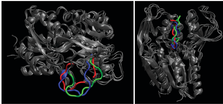
Figure S1 The superimposed structures of LCAT showing the conformation of the lid-region in the X-ray structure of 5TXF (red), before (blue) and after (green) LCAT-water-closed-AA simulation, respectively.
