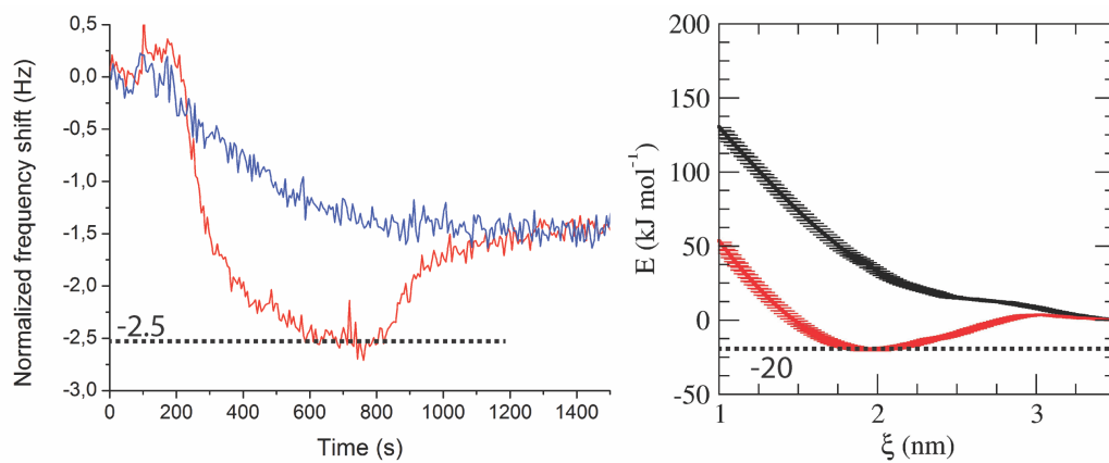
Figure S3 Left: QCM result for the peptide 135-155 (Left). Blue and red curves indicate the pure LCAT and combined LCAT+peptide measurements, respectively. The minimum response is marked with the black dashed line. Right: Potential mean force profiles for the peptide 135-155 with the coil (black) and \alpha -helical secondary structure (red).
