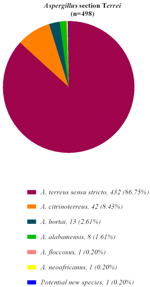
Supplementary Figure S1. Results of molecular identification (partial beta-tubulin sequencing)
